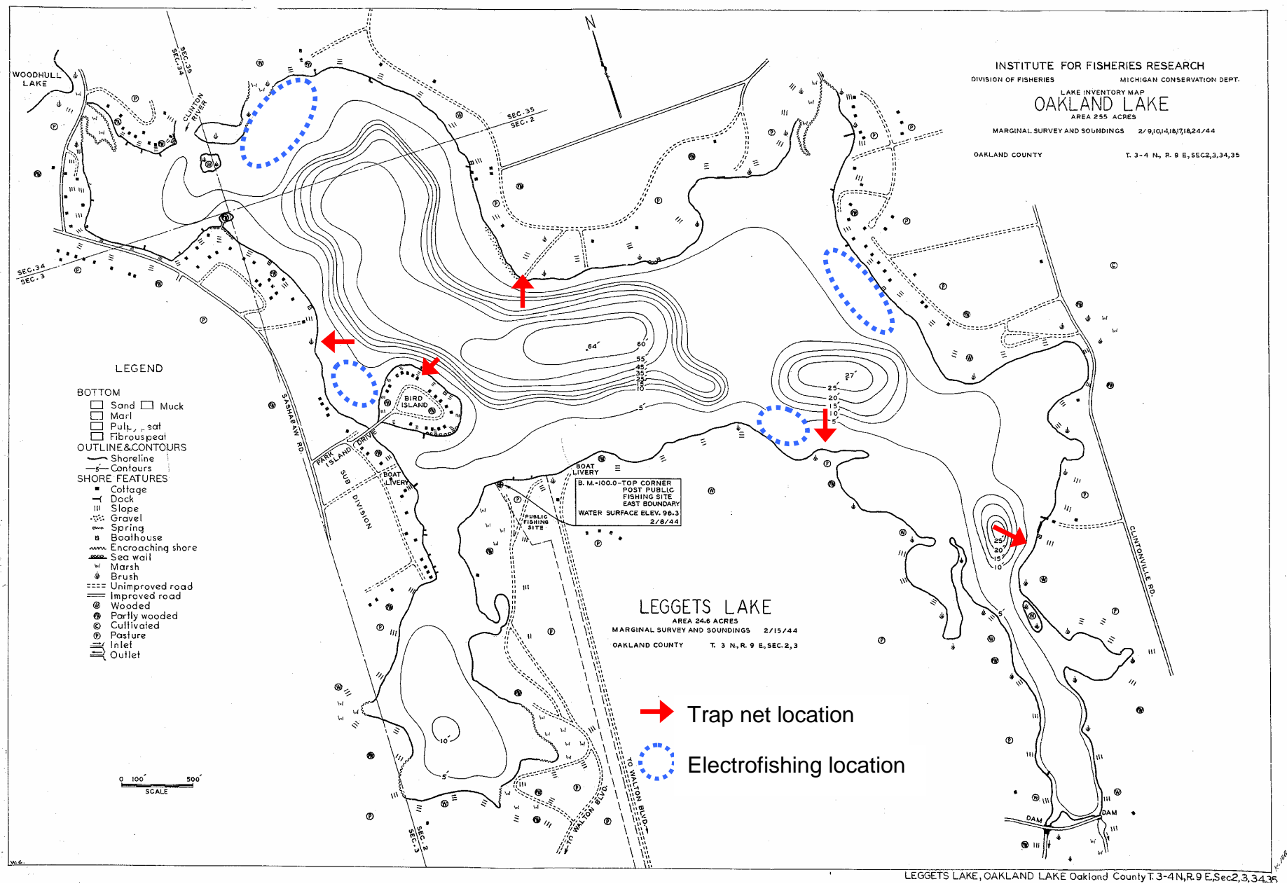
Figure 1.-Map of Oakland Lake with sampling locations.
