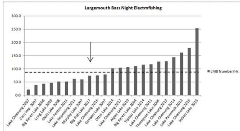
Figure 3. Comparison of night electrofishing catch data for Largemouth Bass in selected waterbodies in southeast Michigan. Dashed line indicated mean value.
