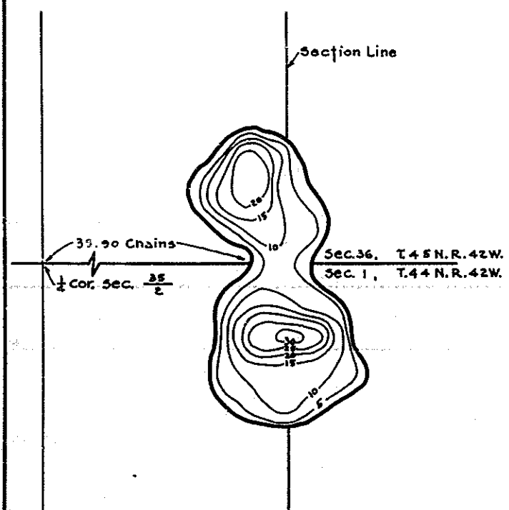
Contour Map Contour Interval = 5'
