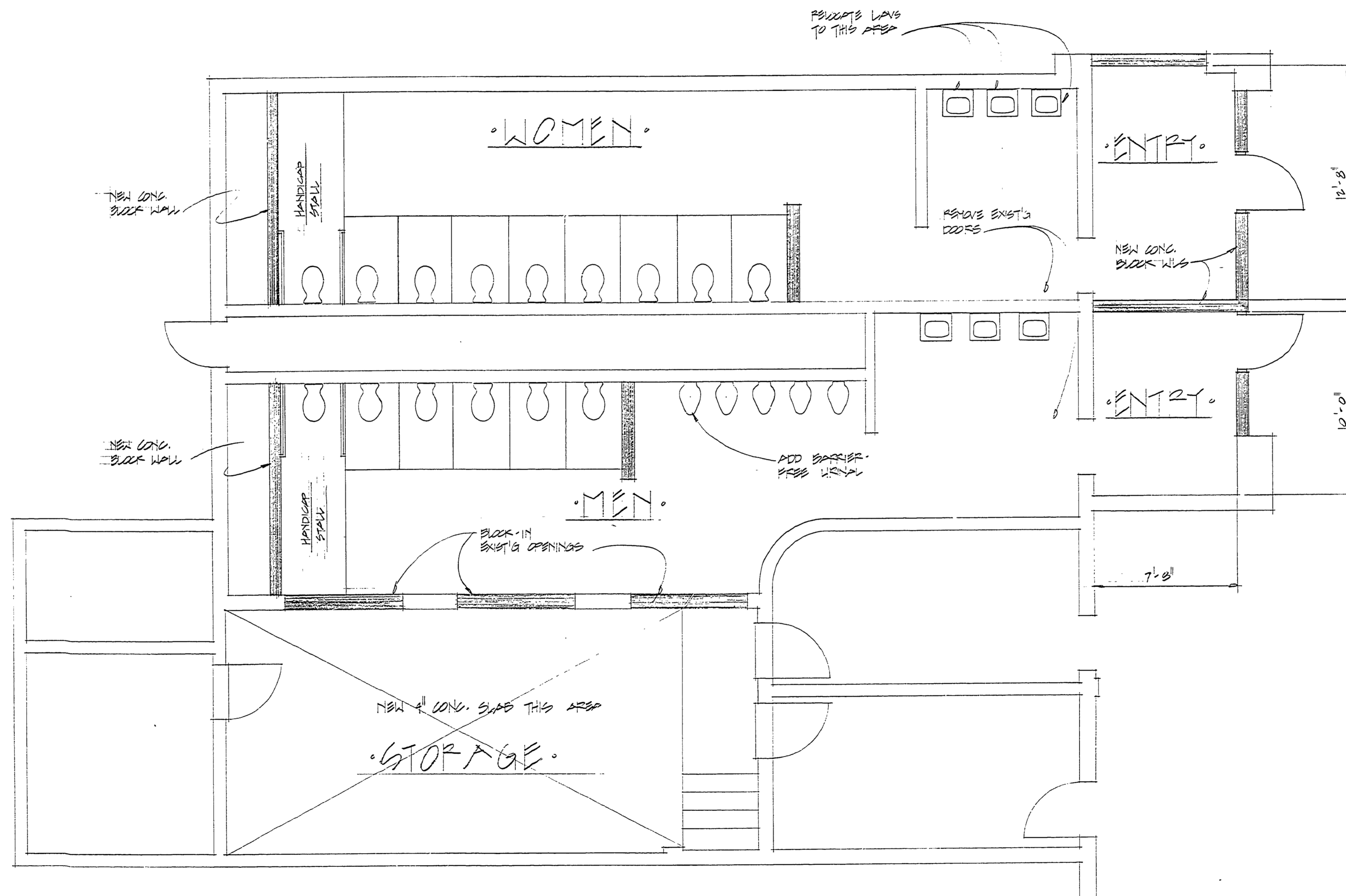
PARTIAL FLOOR PLAN - SOUTH END OF BATHHOUSE 1/4" = ONE FOOT
