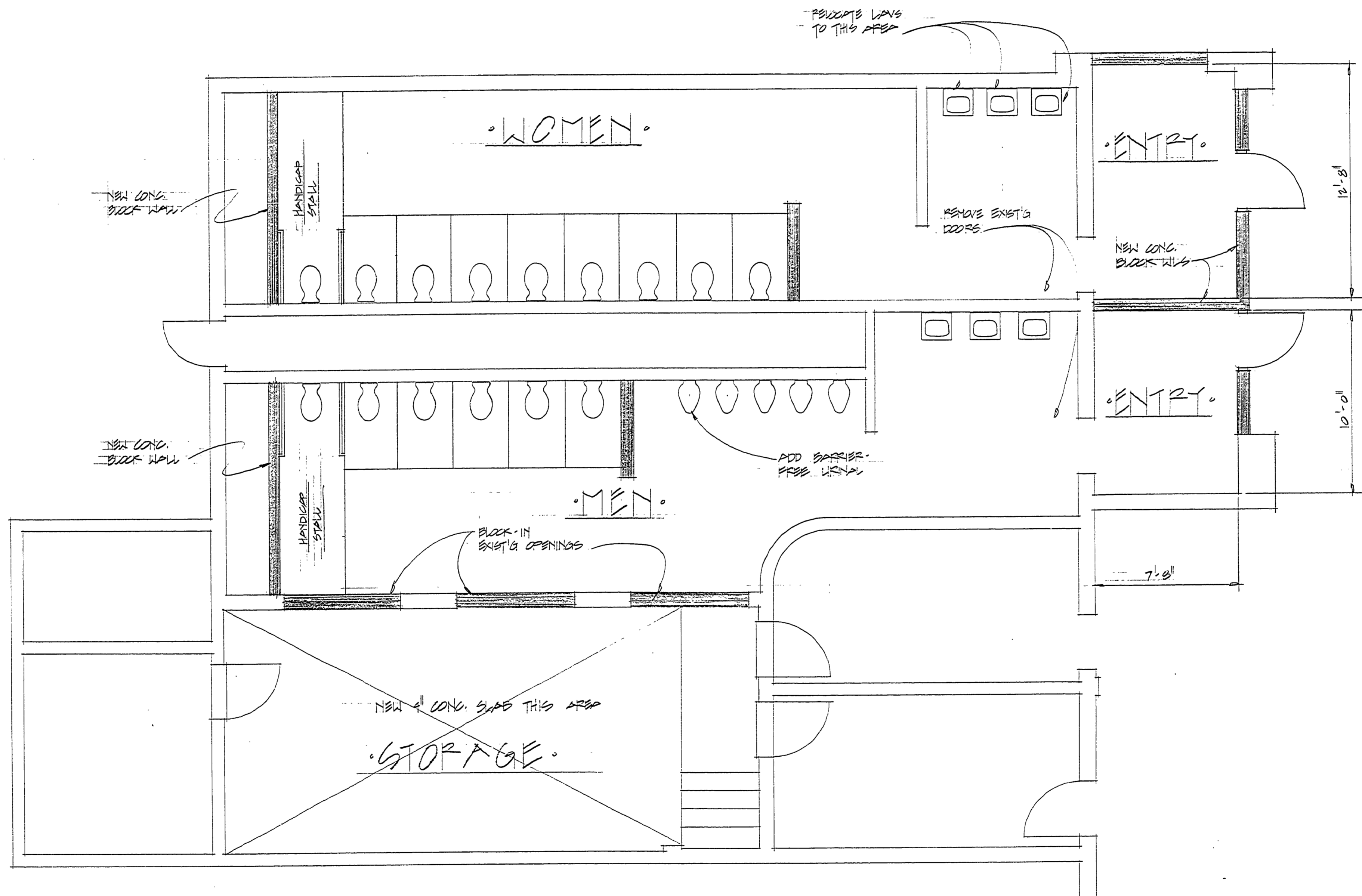
PARTIAL FLOOR PLAN - SOUTH END OF BATHHOUSE. 1/4" = 0'10" FOOT
