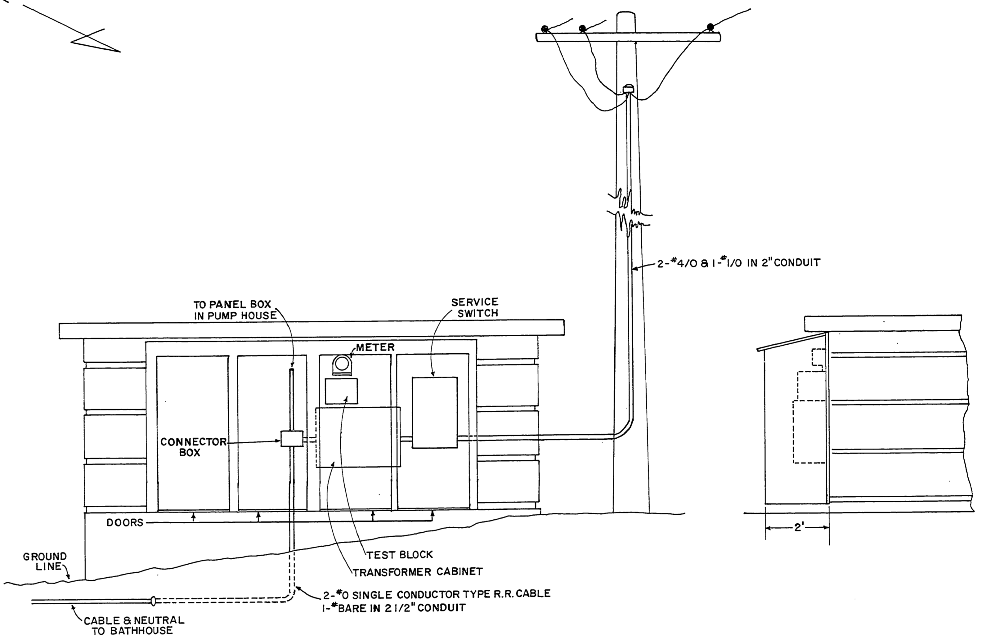
PANEL BOARD SHELTER FRONT ELEVATION SIDE ELEVATION
