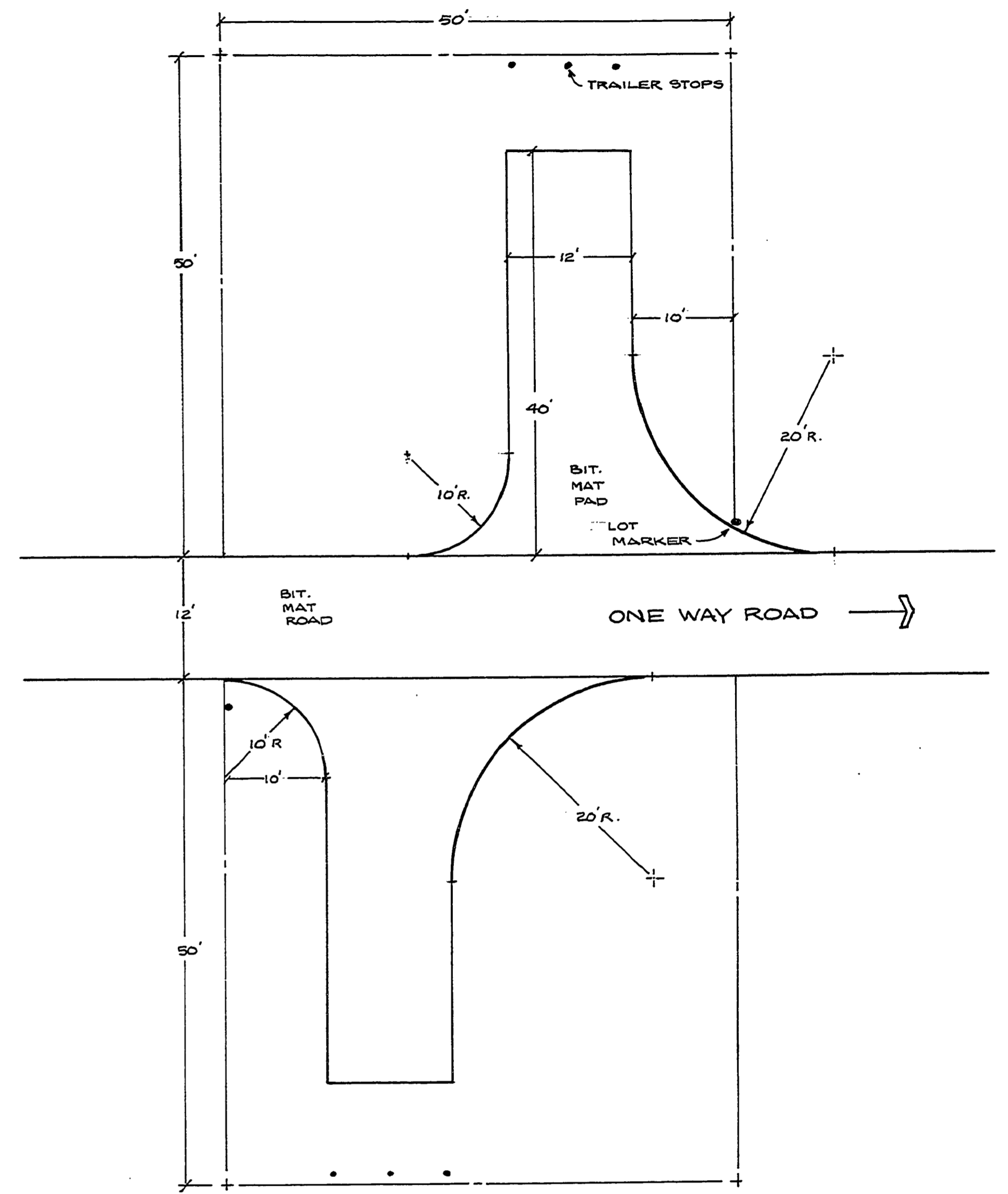
CAMPSITE DETAIL SCALE 1"=10' NOTE: THIS TYPICAL CAMPSITE MAY HAVE TO BE ADJUSTED SLIGHTLY TO FIT UNUSUAL SITE CONDITIONS.
