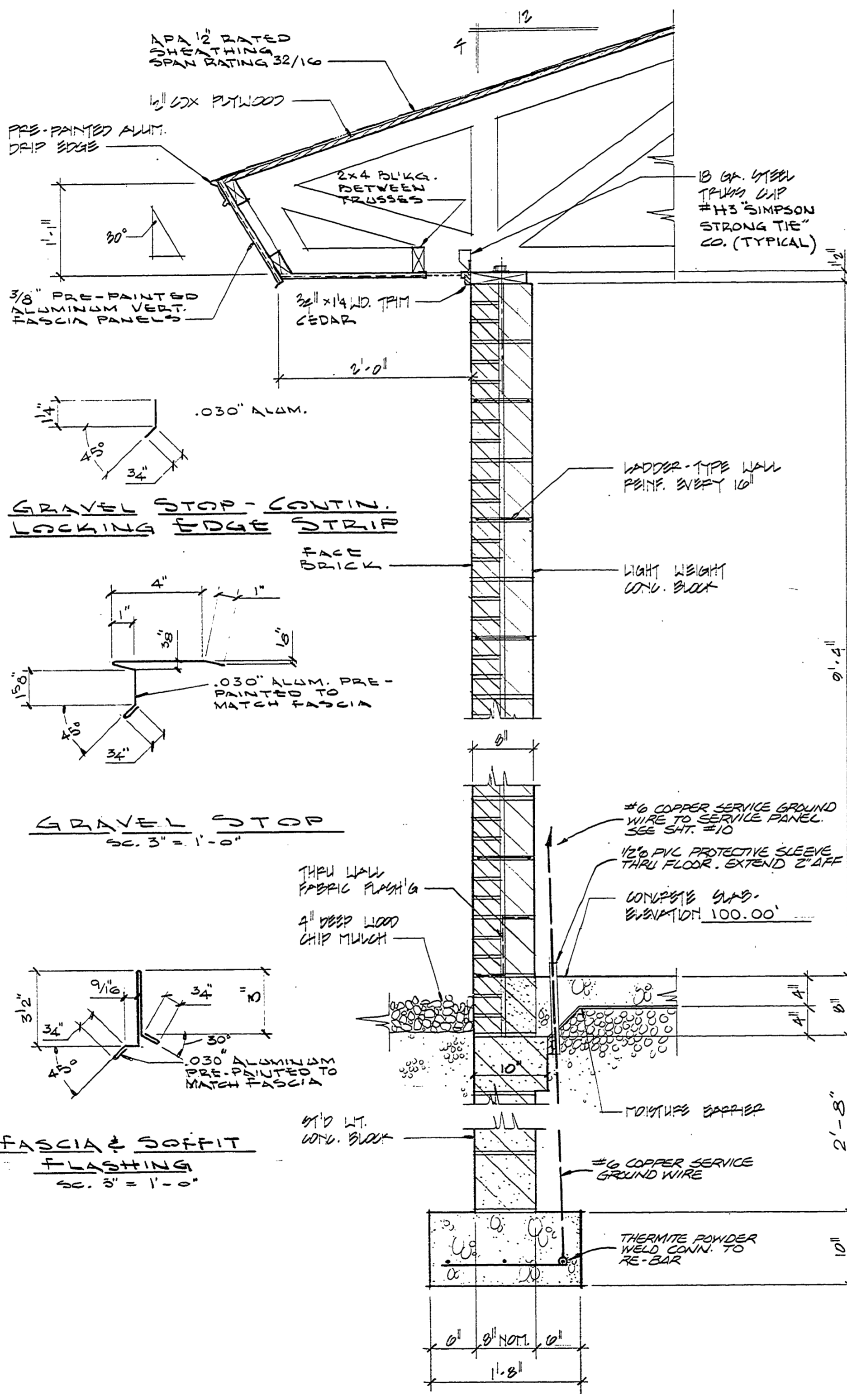
WALL SECTION 8 5/8
