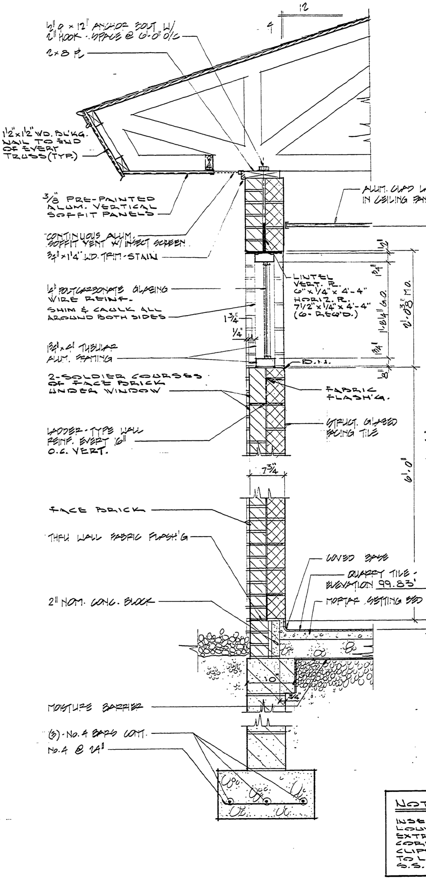
WALL SECTION 9 5/8
