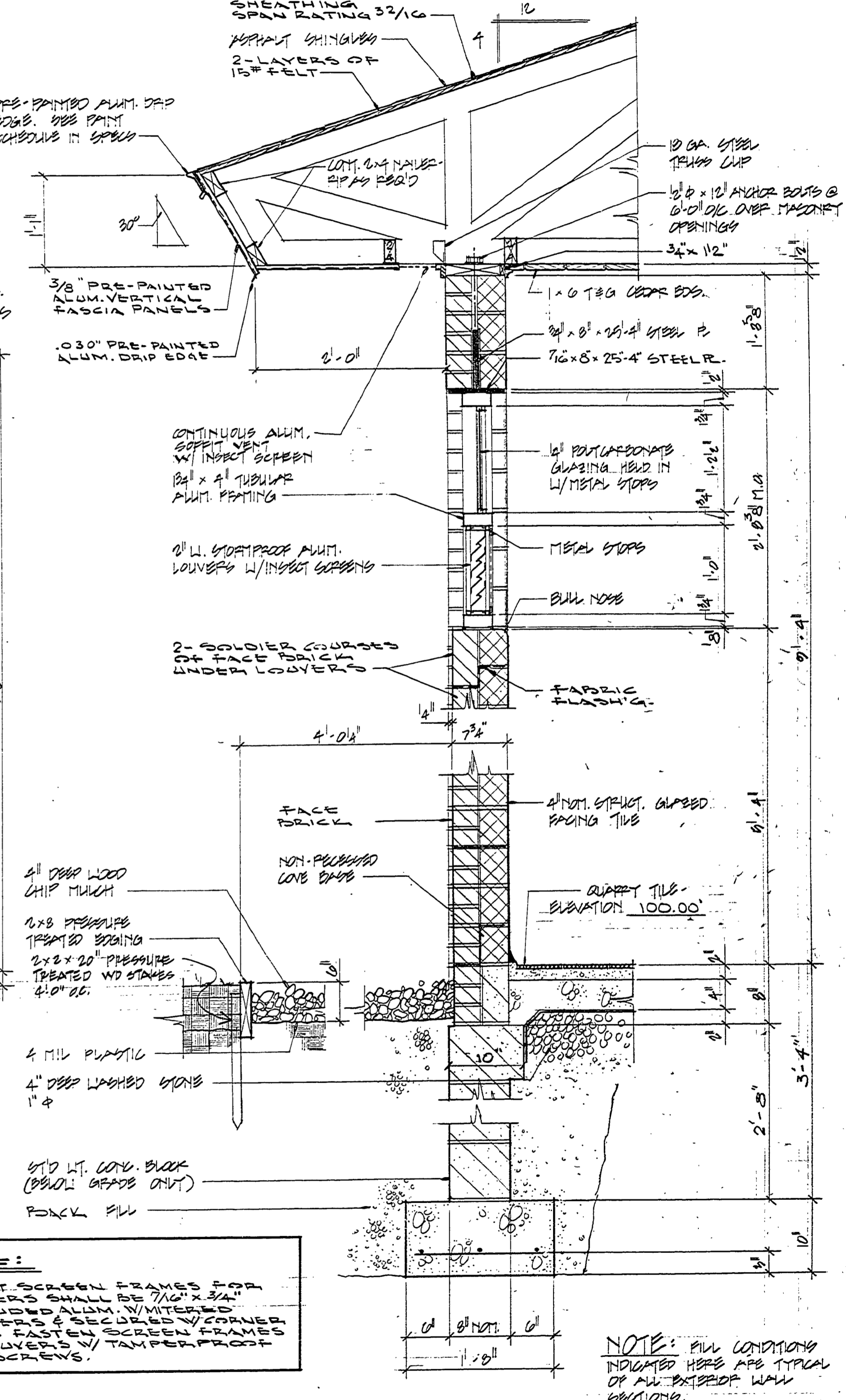
WALL SECTION 10 5/8
