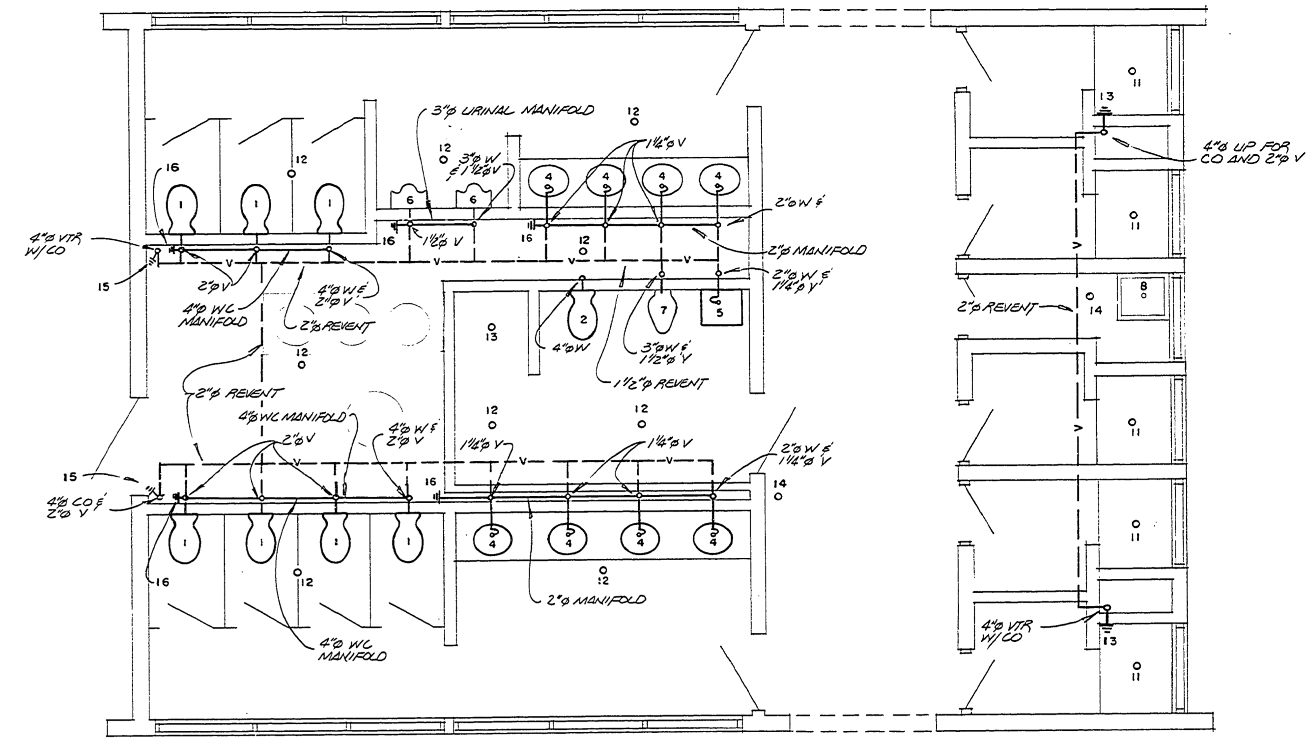
ABOVE SLAB WASTE PLUMBING PLAN SCALE 1/4" = 1'-0"
