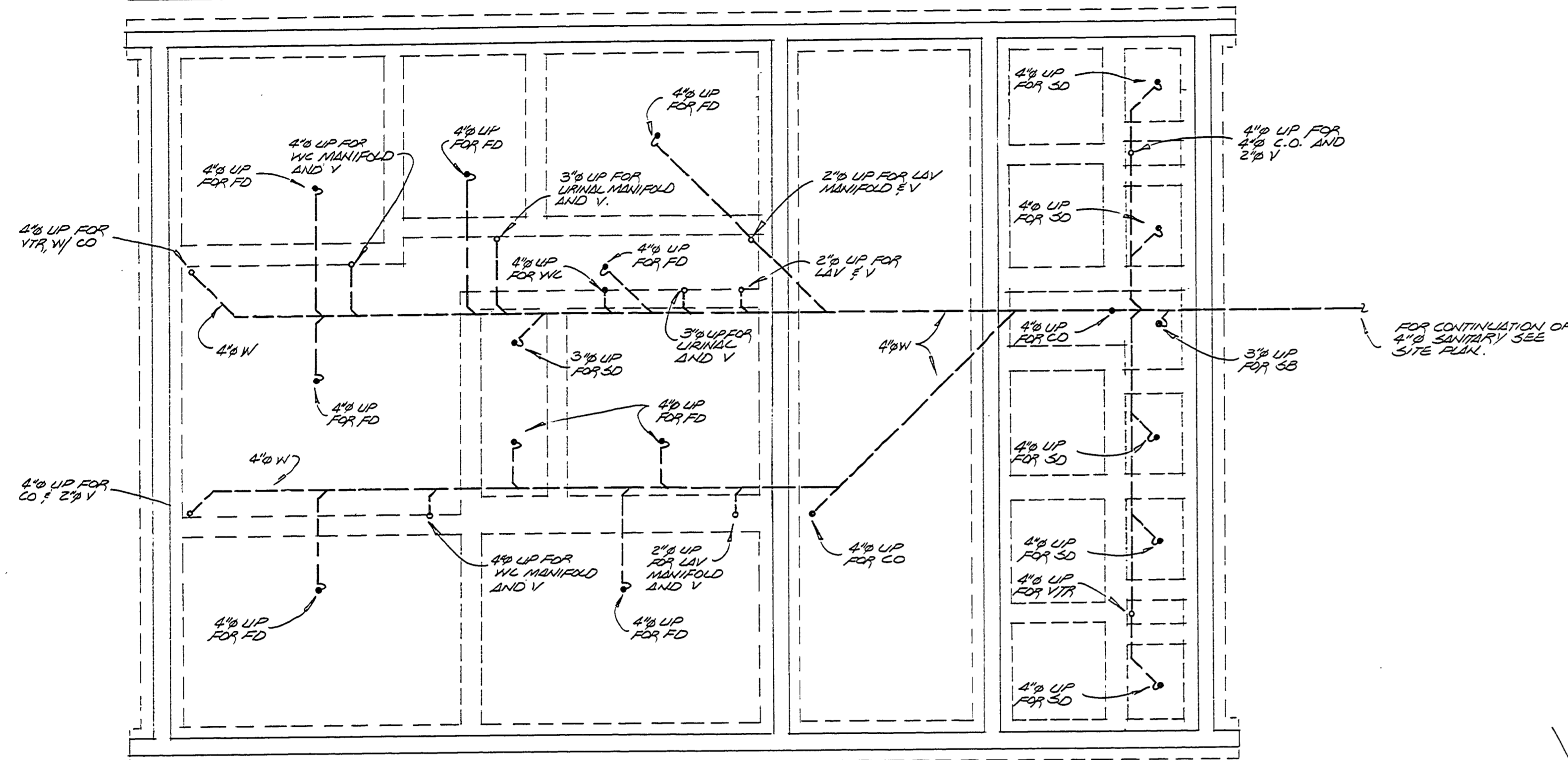
BELOW SLAB WASTE PLUMBING PLAN SCALE 1/4" = 1'-0"
