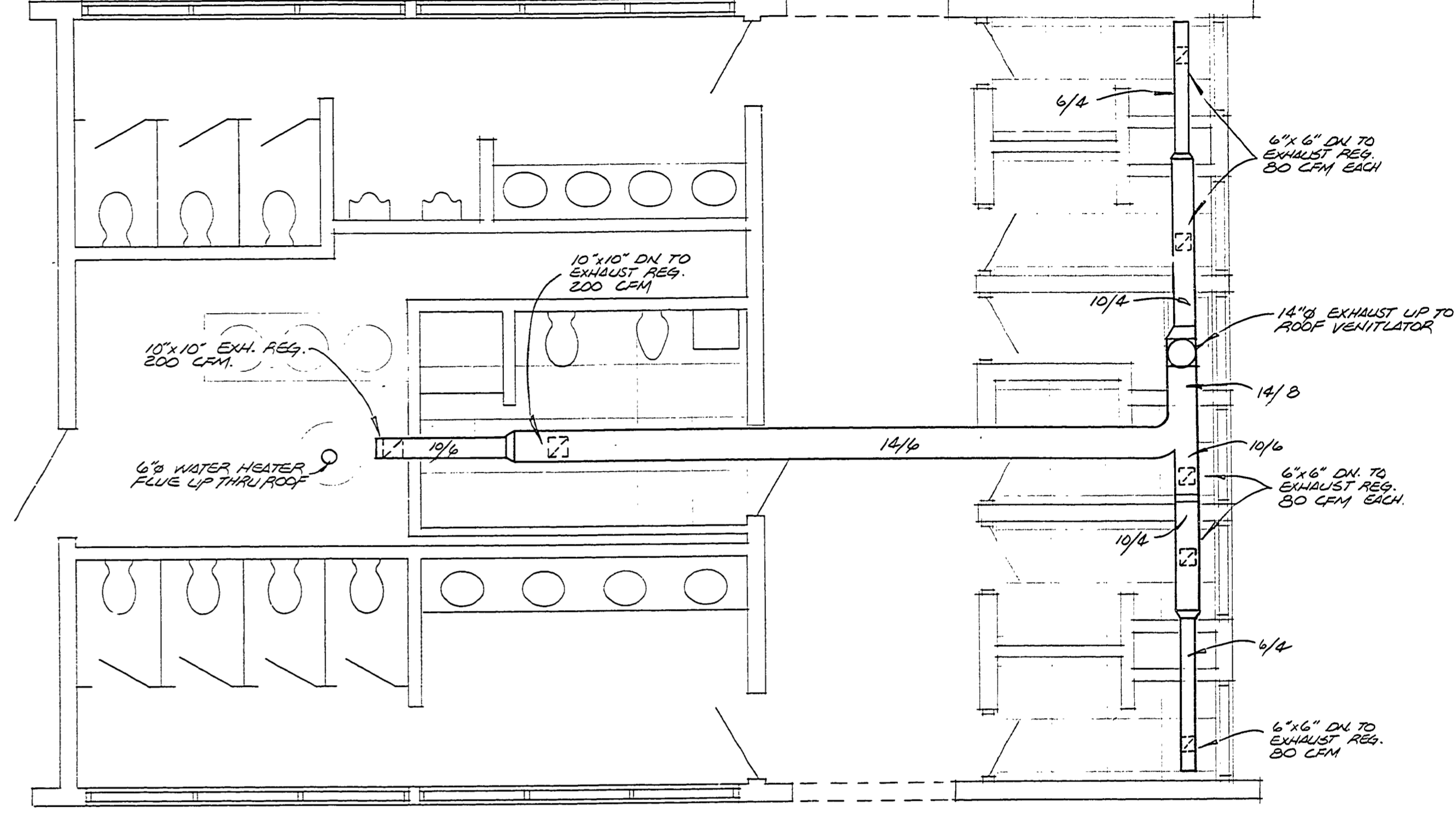
VENTILATION FLOOR PLAN SCALE 1/4" = 1'-0"
