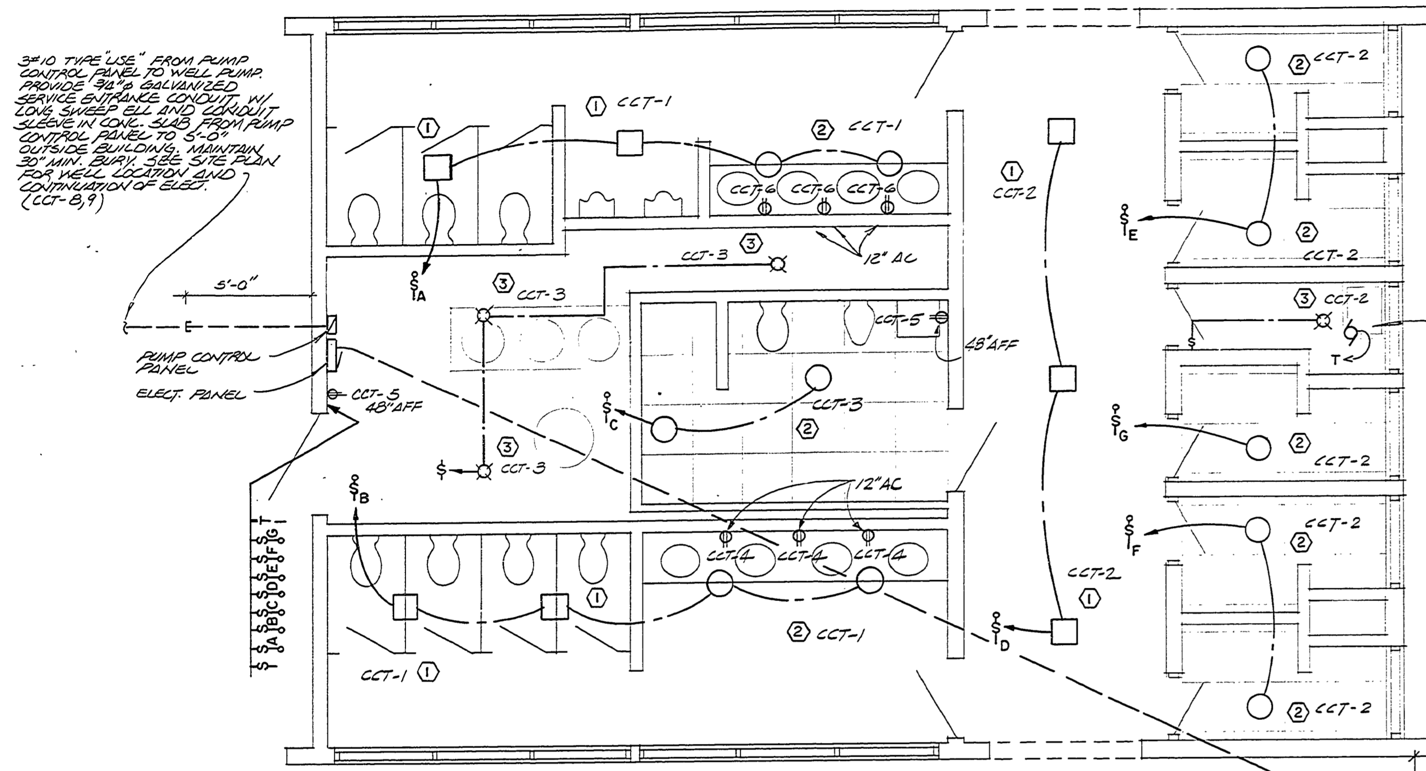
ELECTRICAL FLOOR PLAN SCALE 1/4" = 1'-0"
