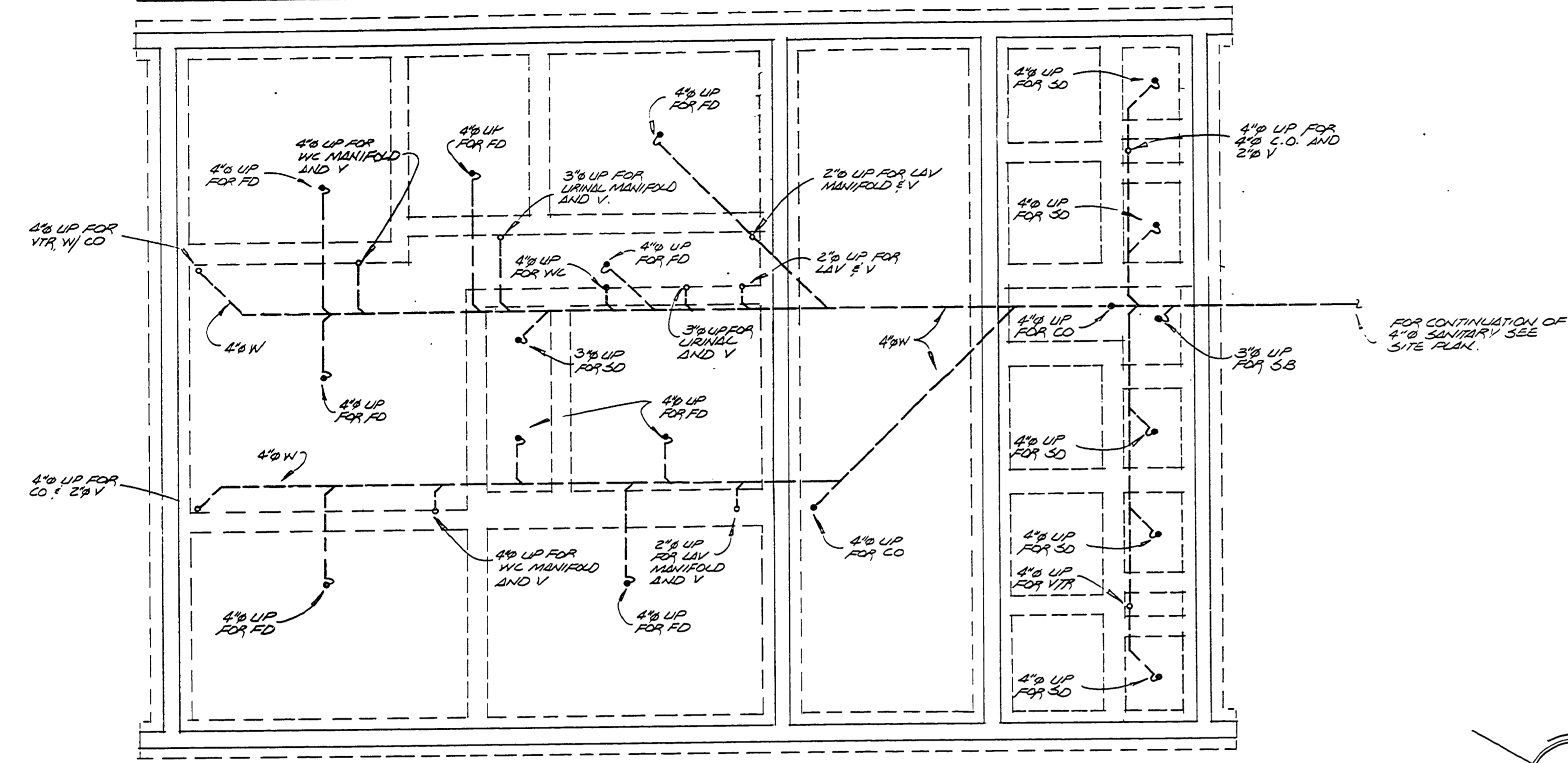
BELOW SLAB WASTE PLUMBING PLAN SCALE 1/8" = 1'-0"
