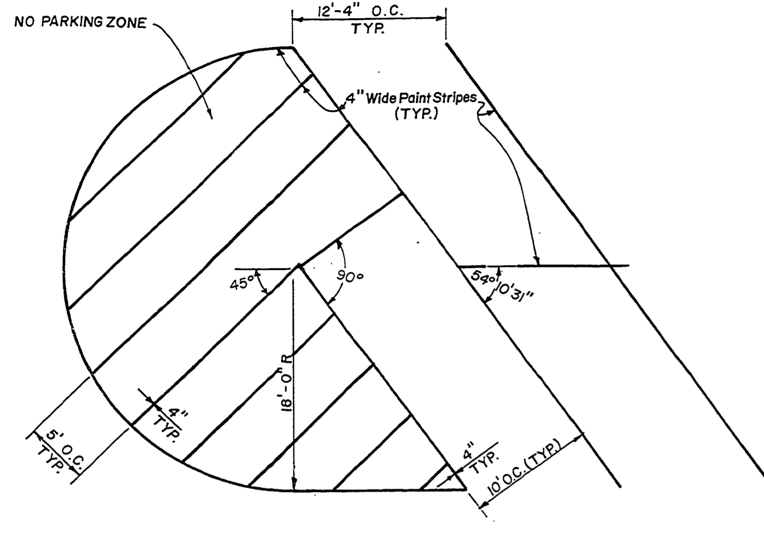
PARKING STALL LAYOUT 1/8" = 1'-0"
