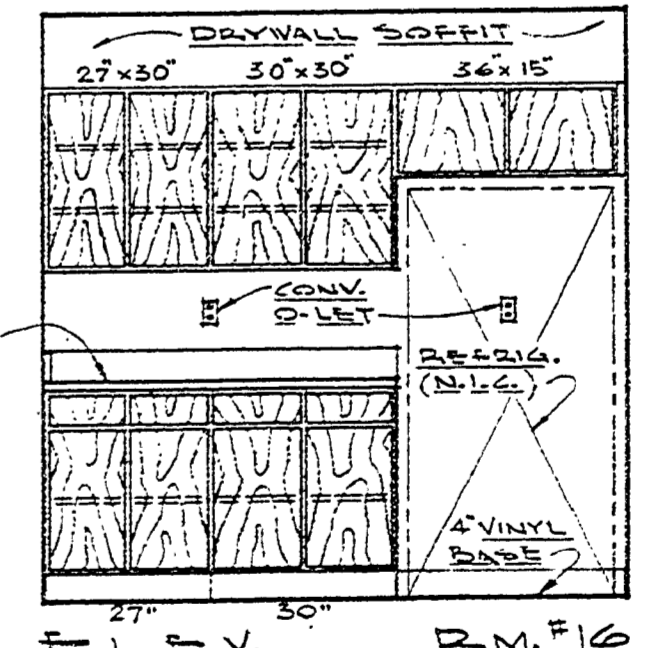
ELEV. R.M.#16 25' 3" x 11'-0"
