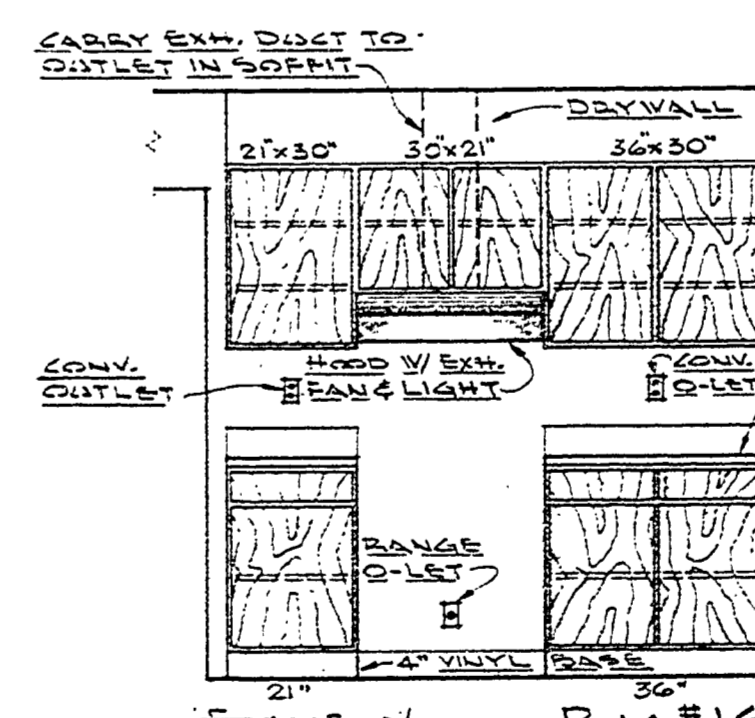
ELEV. R.M.#16 25' 3" x 11'-0"
