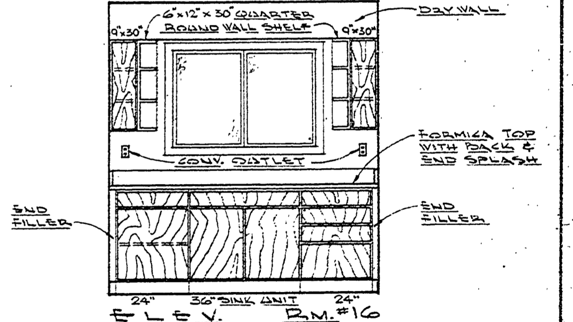
ELEV. R.M.#16 25' 3" x 11'-0"
