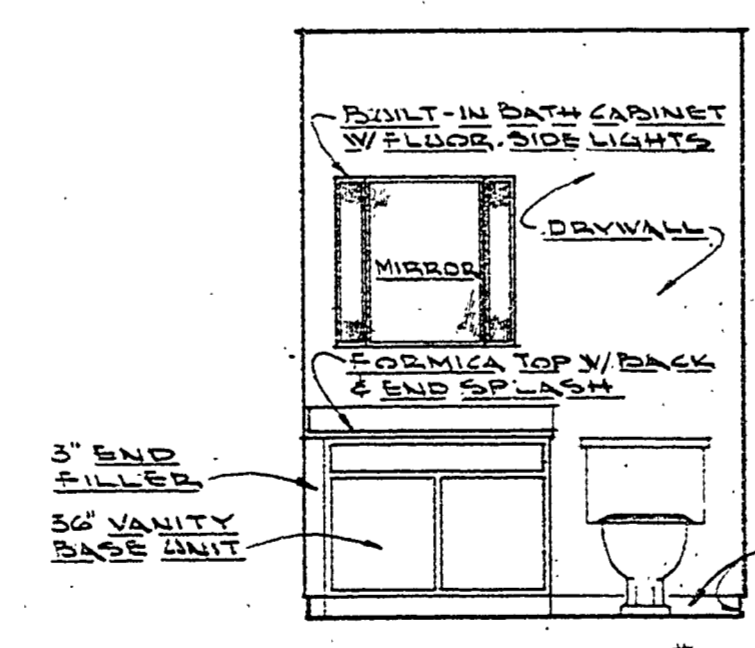
ELEV. R.M.#13 25' 3" x 11'-0"
