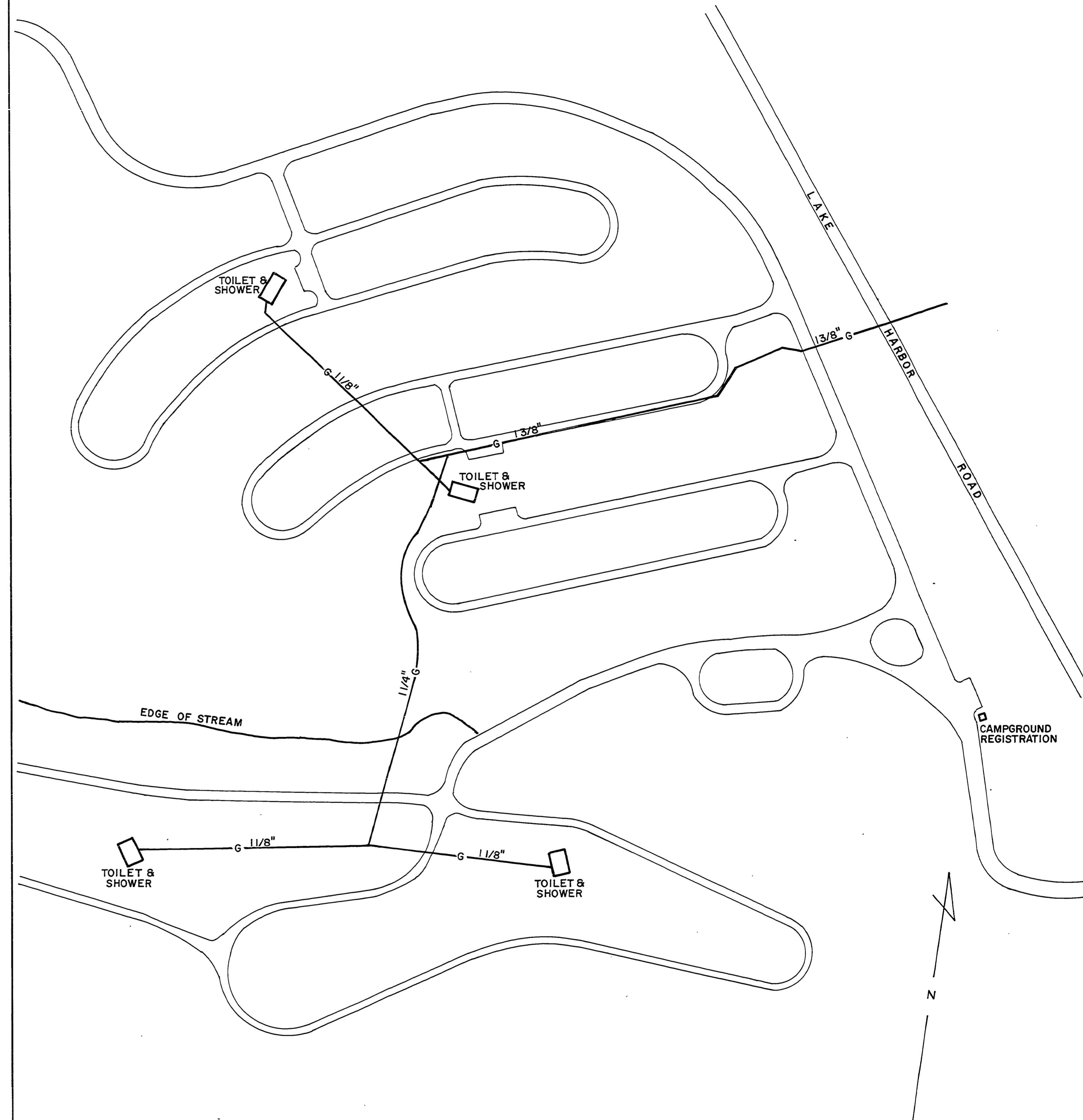
PLASTIC GAS LINE-NATURAL GAS
