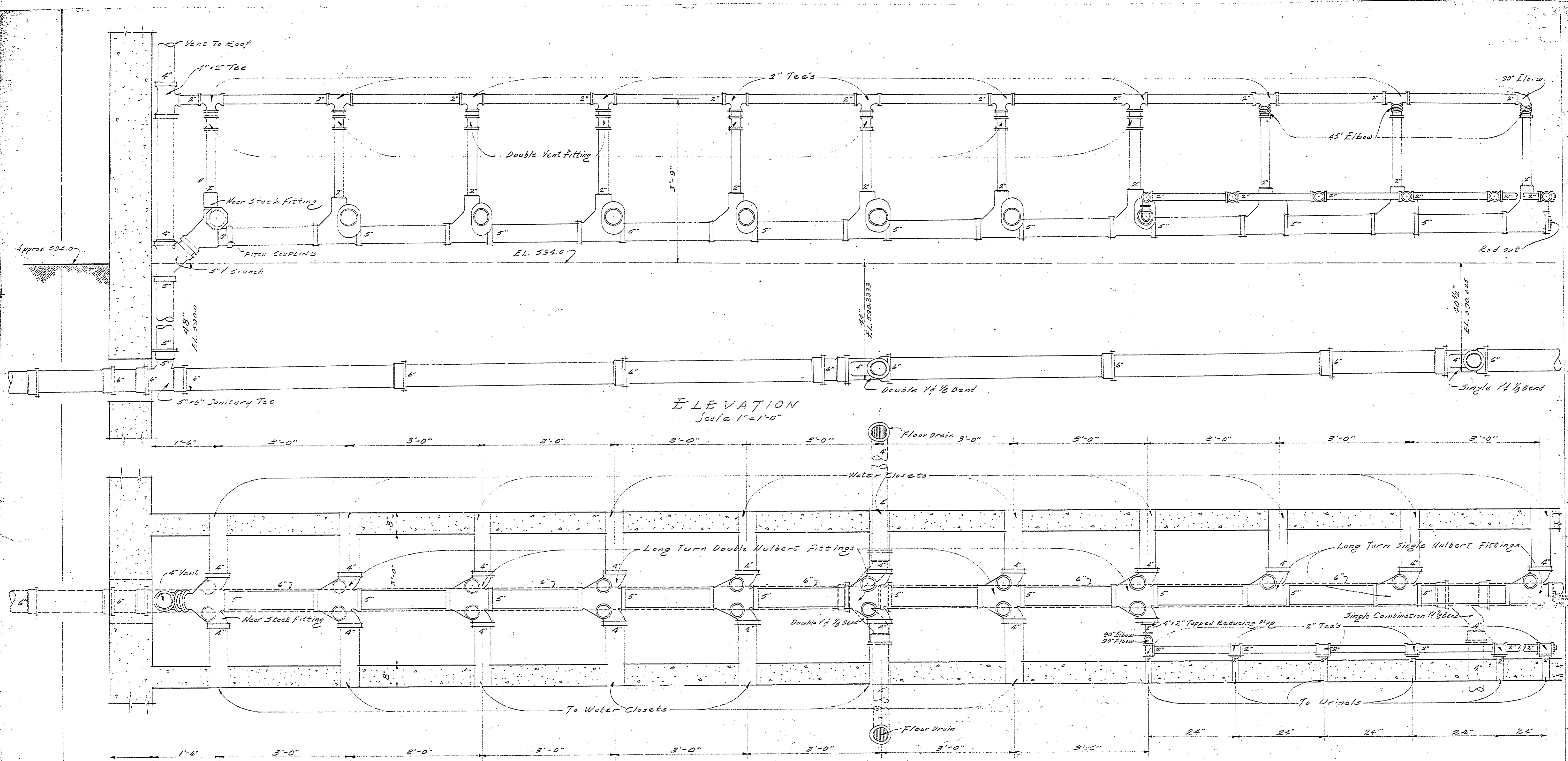
PLAN OF PLUMBING THROUGH MAIN PIPE CHAMBER Scale 1" = 1'-0"
