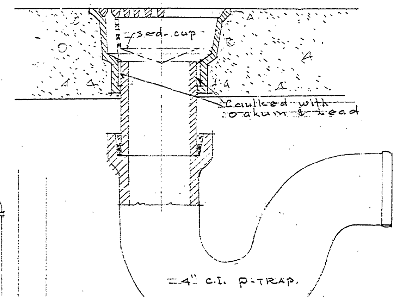
DETAIL OF SHOWER FLOOR DRAINS SCALE 3/4" = 1'-0"
