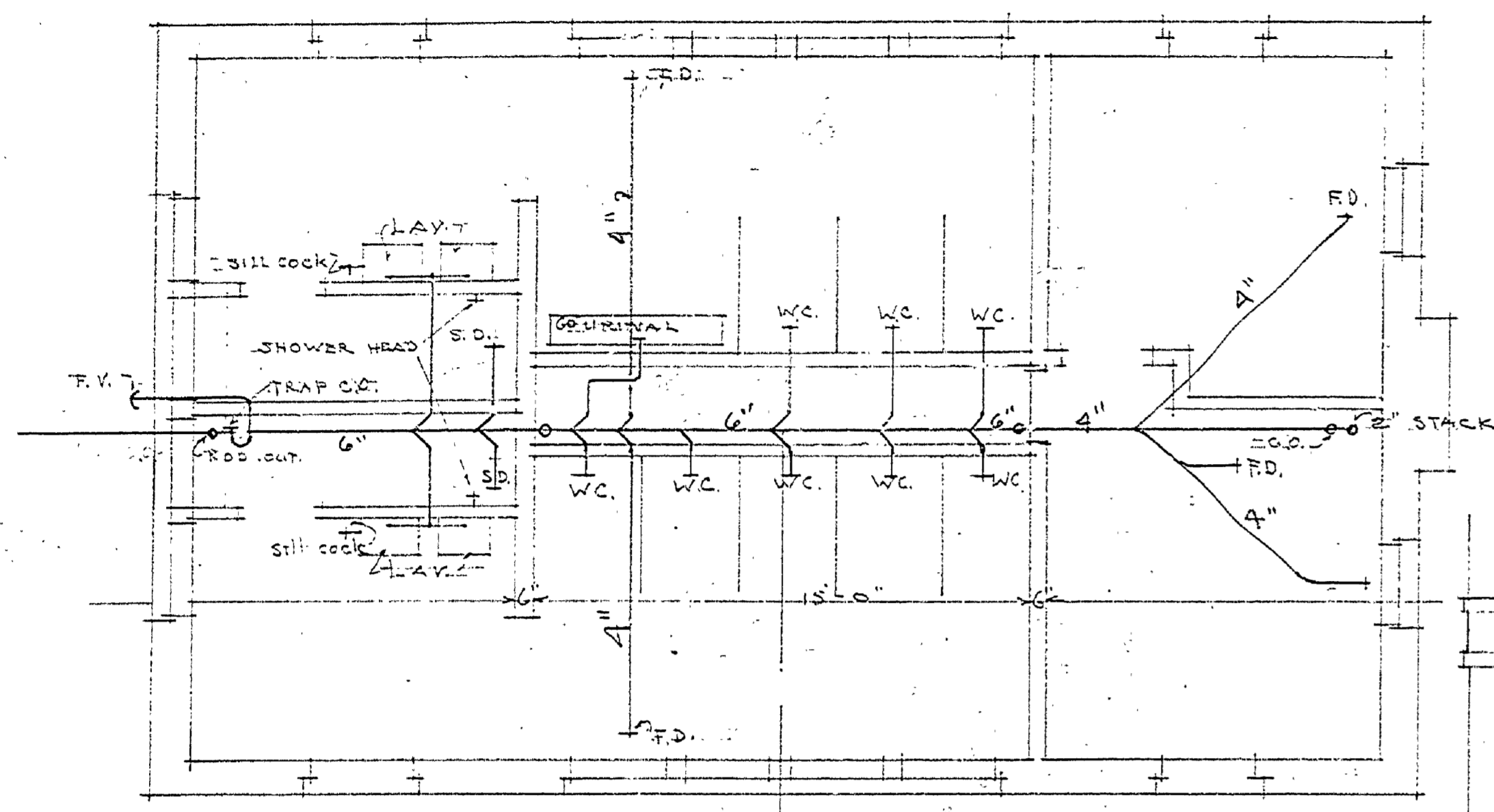
LAY OUT OF DRAINAGE SCALE 1/4" = 1'-0"
