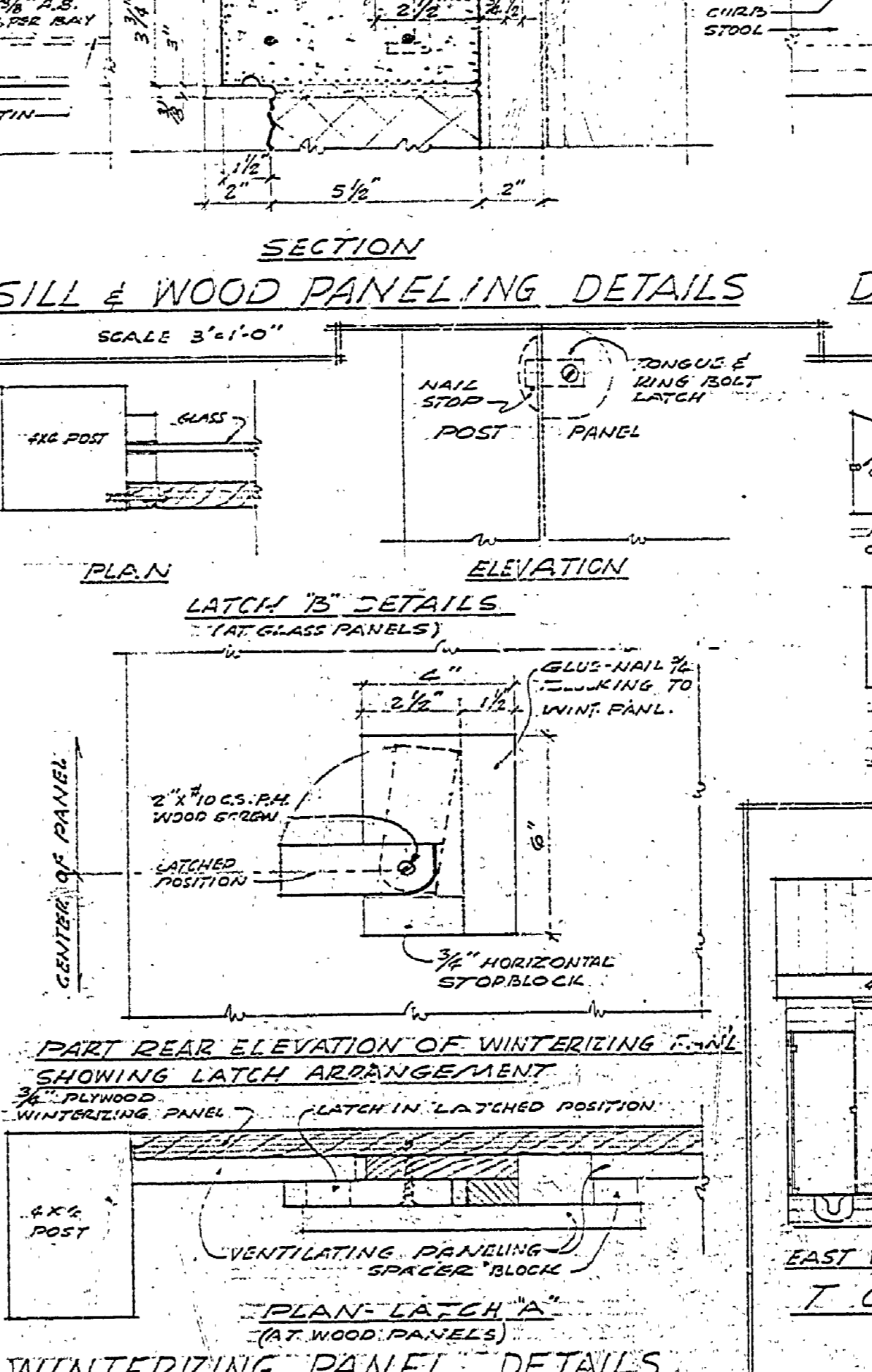
WINTERIZING PANEL DETAILS SCALE 3" = 1'-0"
