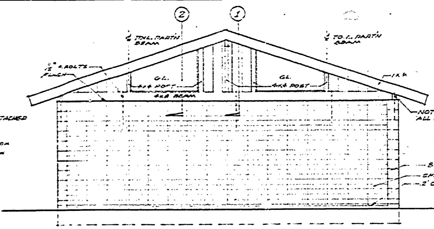
NORTH ELEVATION
