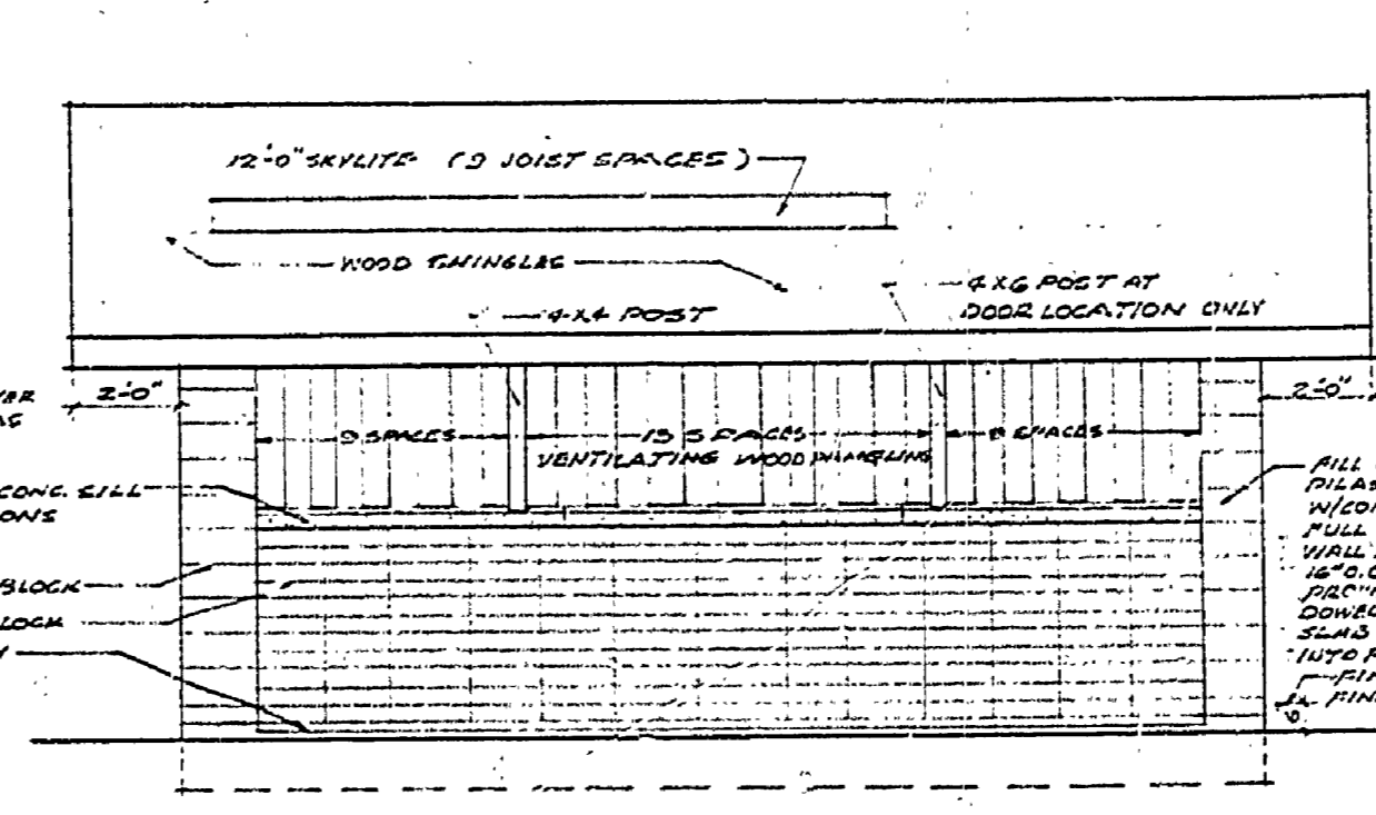
WEST ELEVATION EAST ELEV. OPP. HAND
