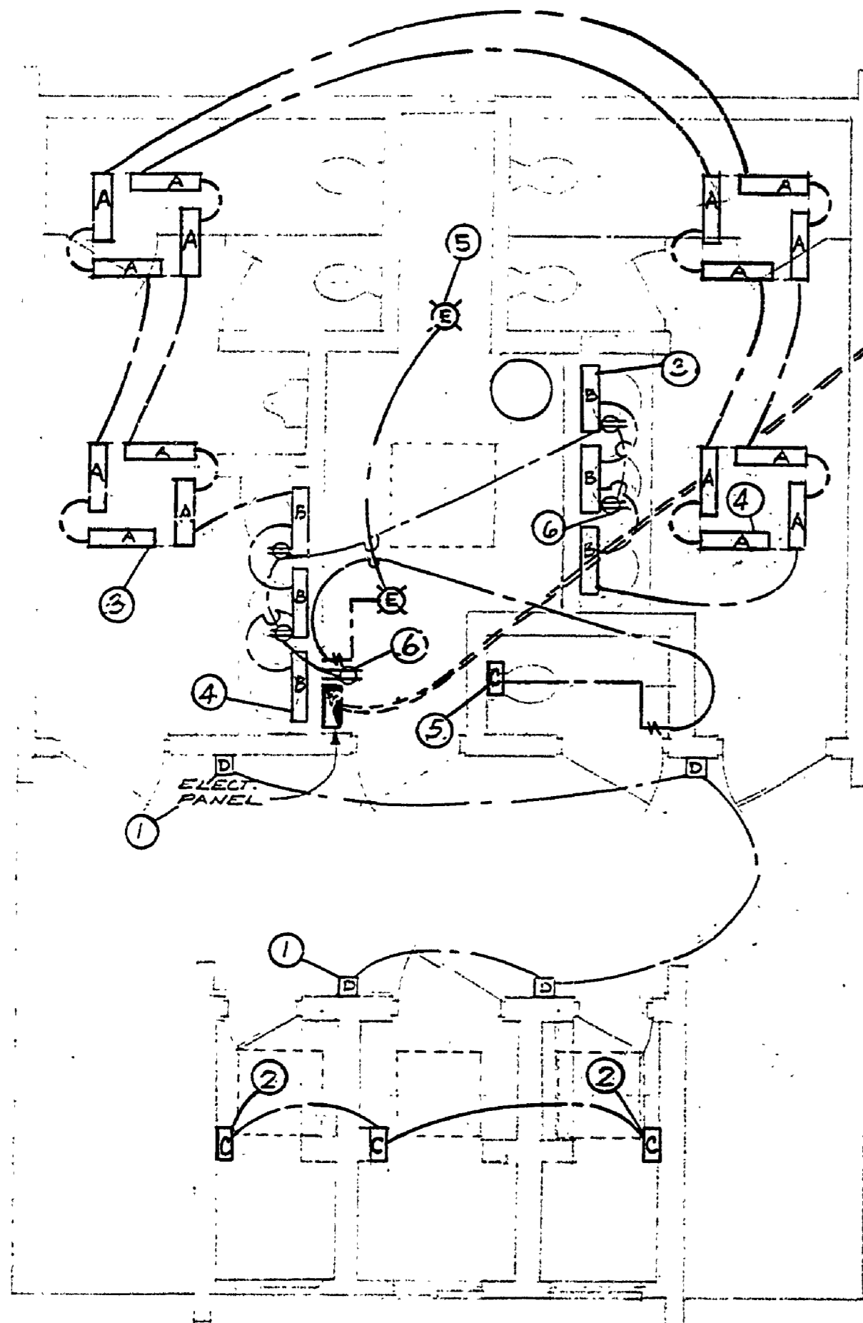
LIGHTING & RECEPTACLE PLAN 1/4" = 1'-0"
