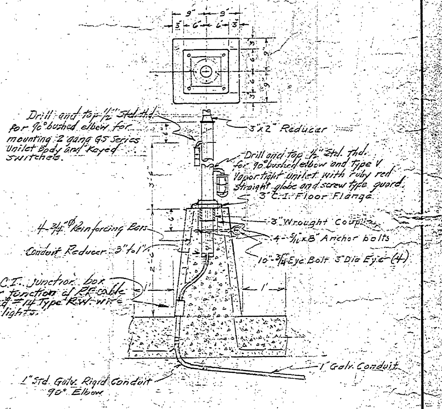
DETAIL OF CONC. BASE SCALE 3/4" = 1'-0"
