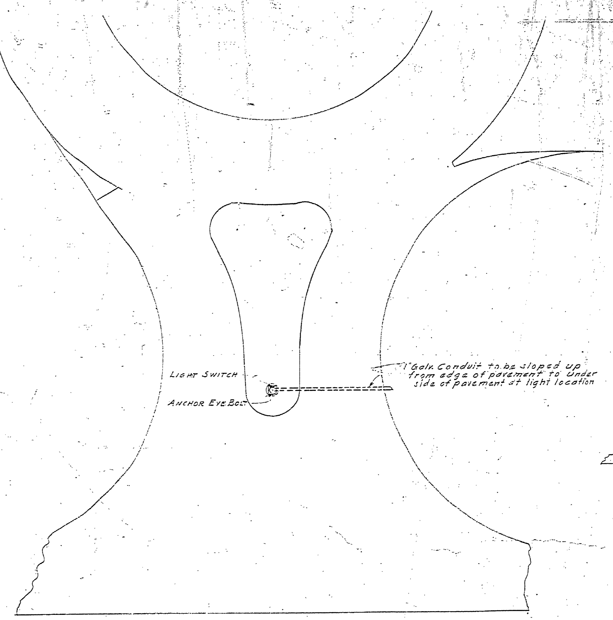
LIGHTING STANDARD DETAILS SCALE 3/8" = 1'-0"
