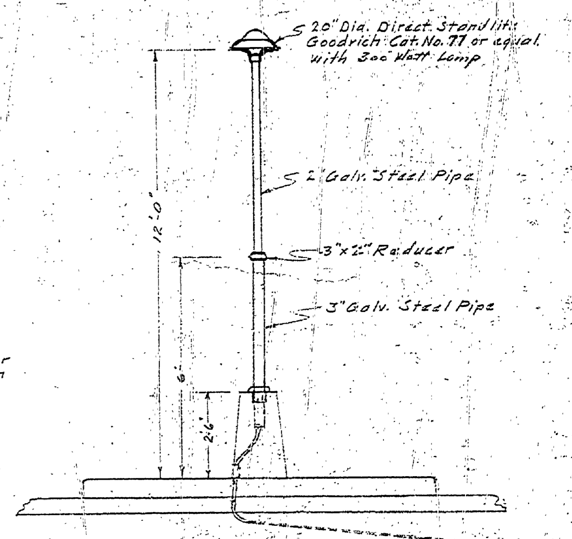
LIGHTING STANDARD DETAILS SCALE 3/8" = 1'-0"
