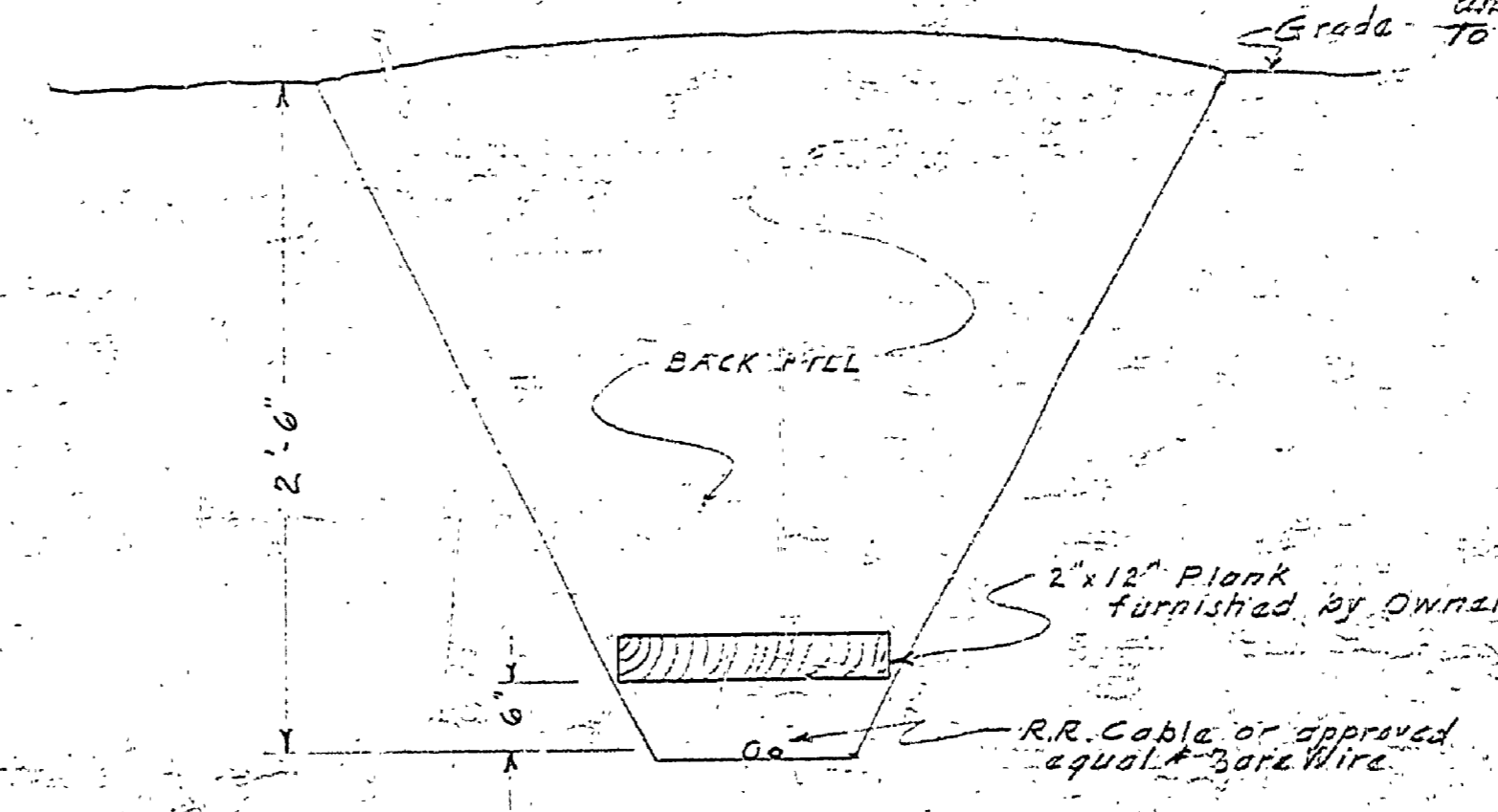
CROSS SECTION OF CABLE TRENCH NO SCALE
