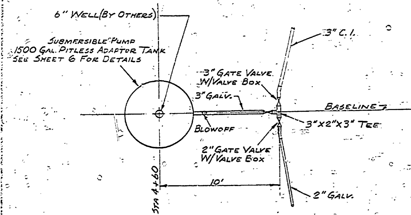
WATER SUPPLY PLAN 1" = 5'
