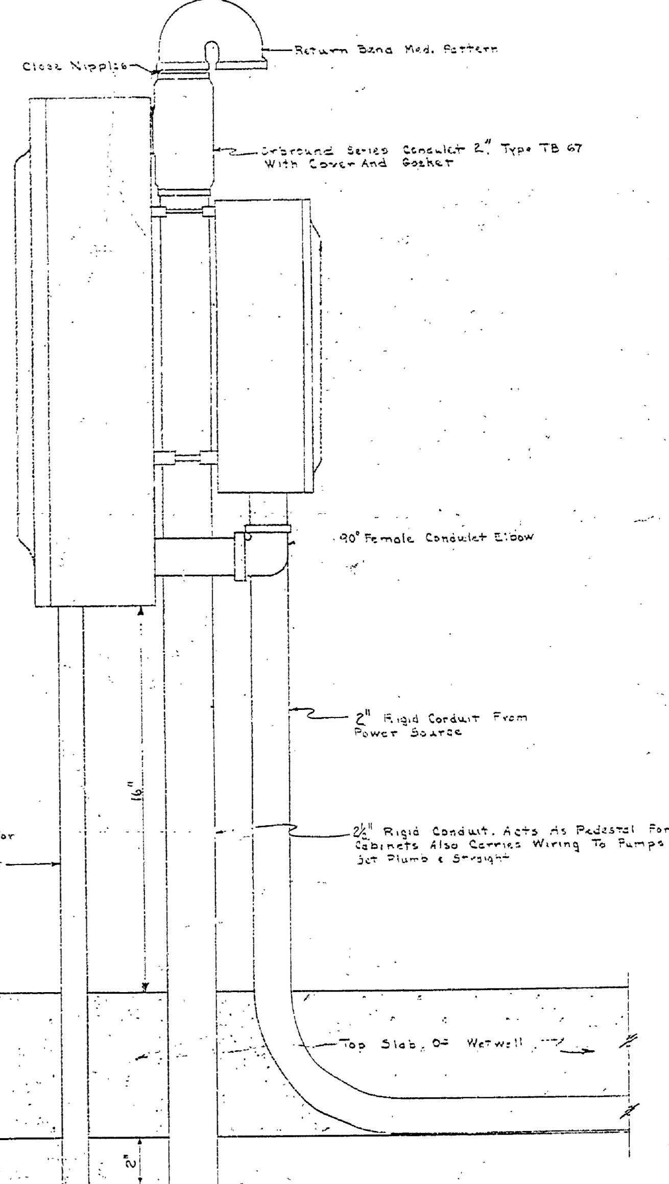
FRONT ELEVATION
