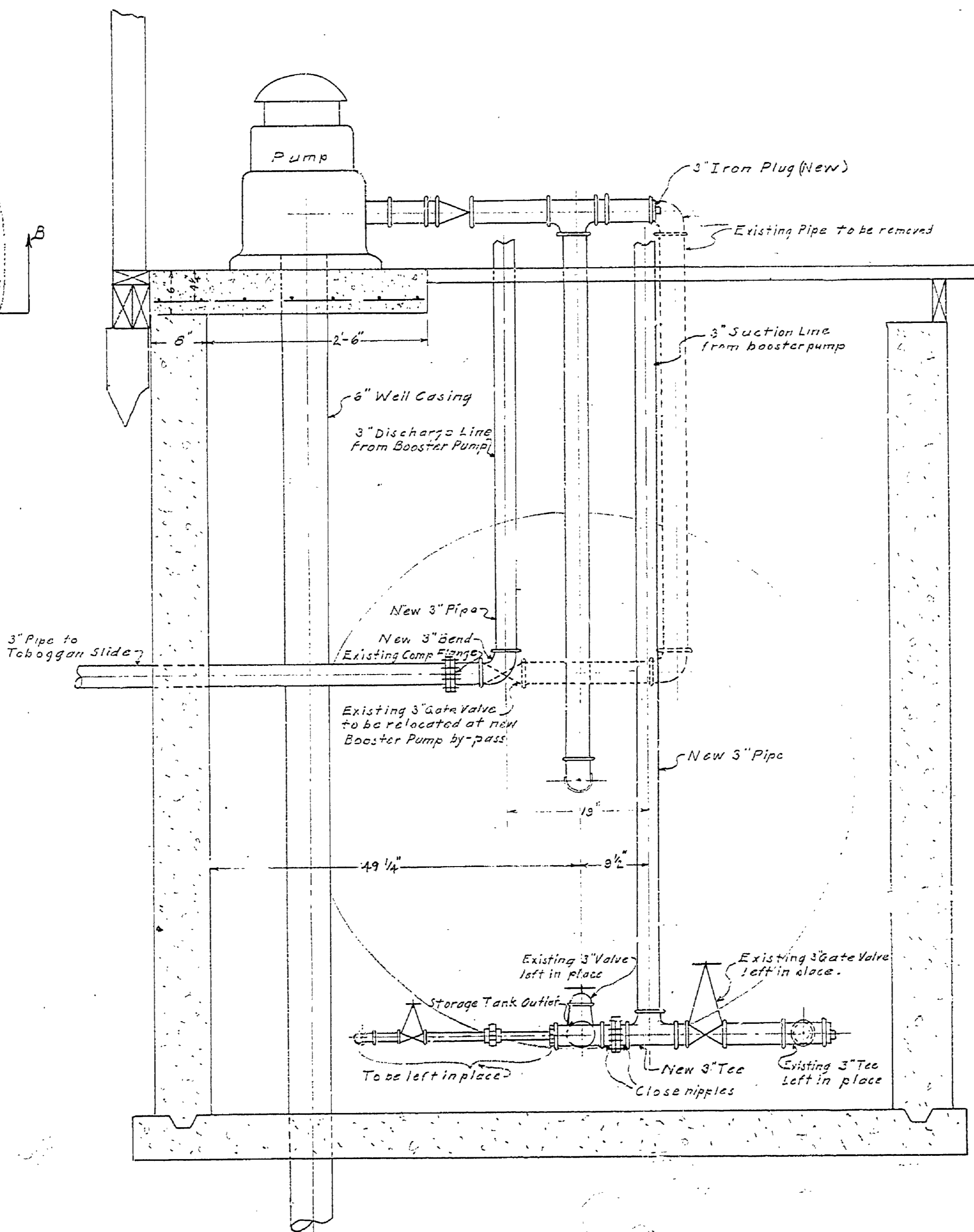
SECTION A-A SCALE 1 1/2"=1'-0"
