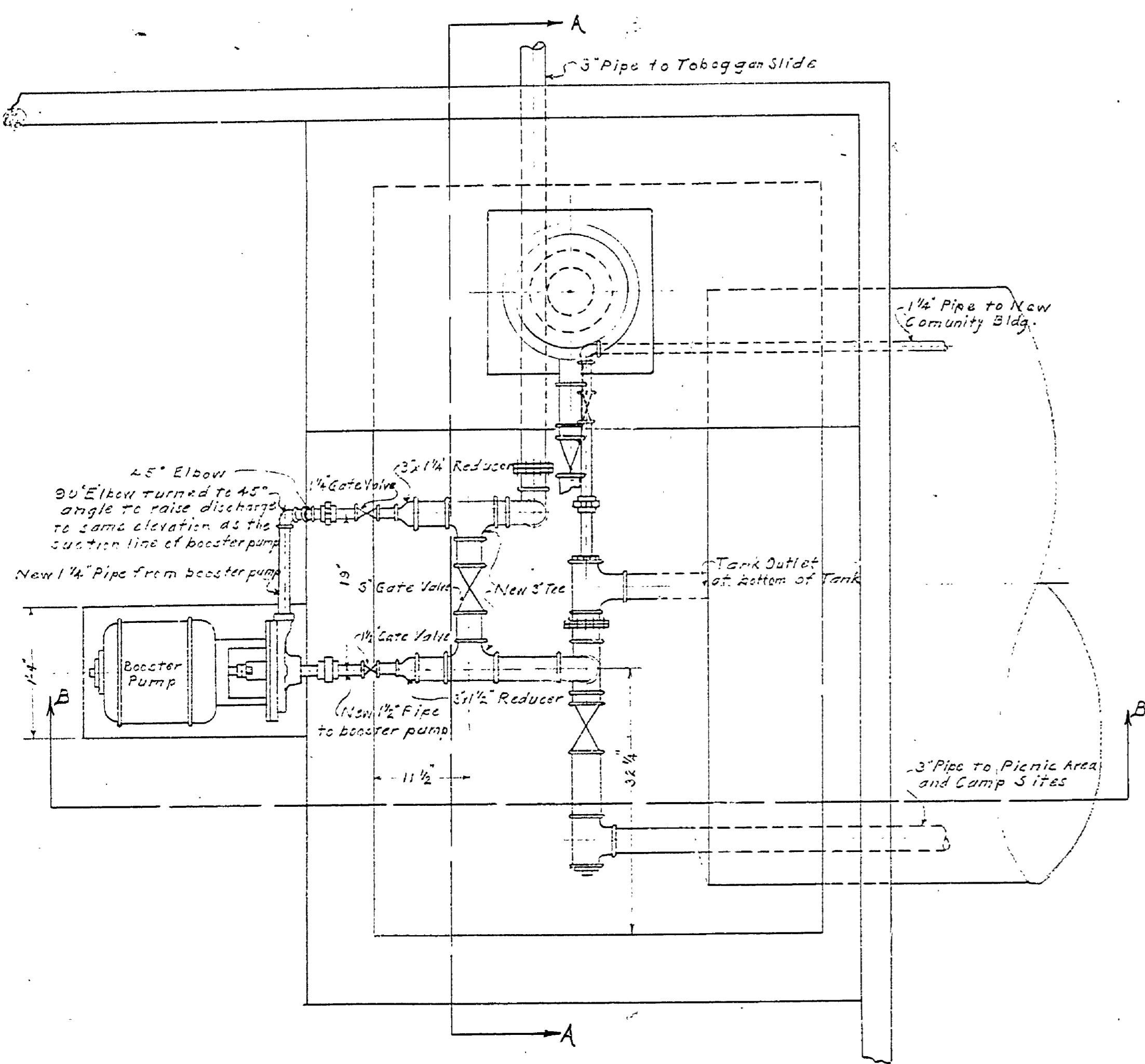
PLAN OF BOOSTER PUMP LAYOUT SCALE 1 1/2"=1'-0"
