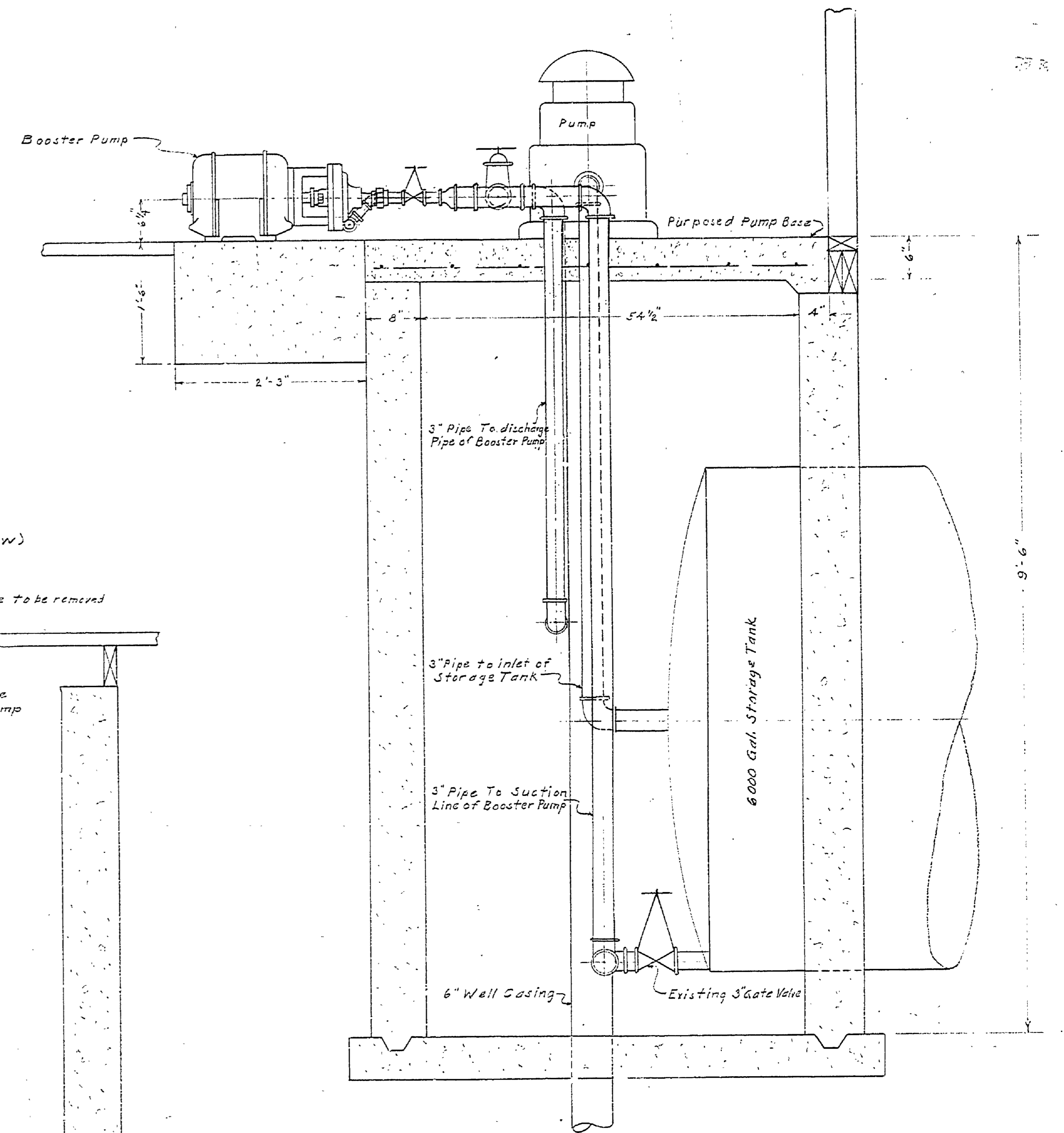
SECTION B-B SCALE 1 1/2"=1'-0"
