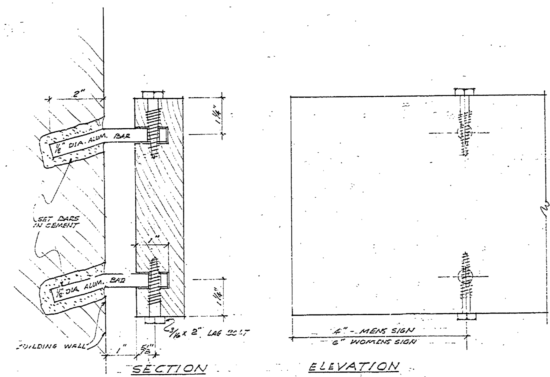
MOUNTING DETAIL SCALE 1/2" = 1'-0"
