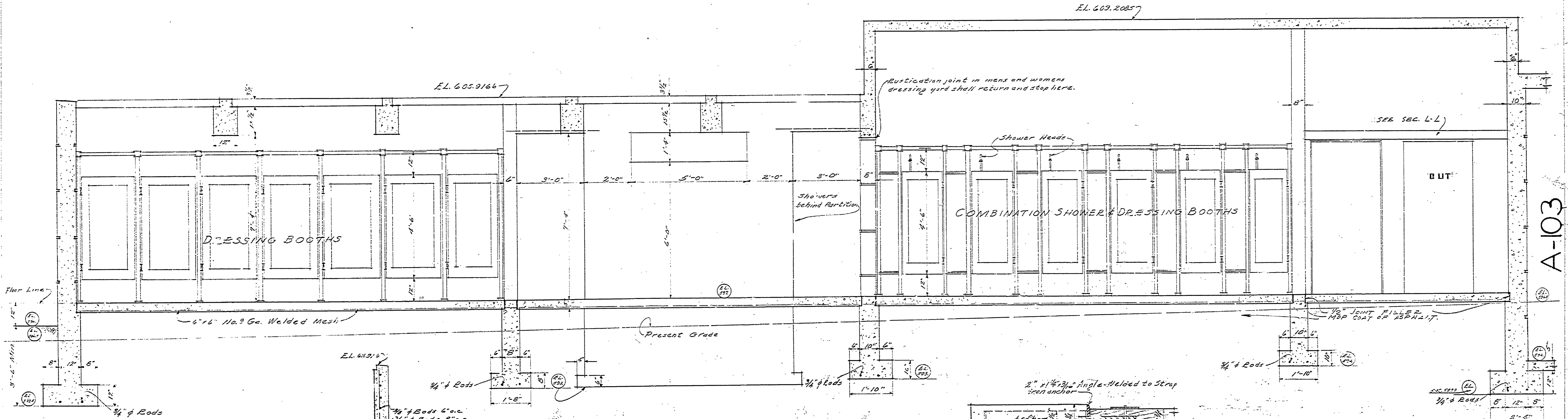
SECTION K-K Scale 1/2"=1'-0"
