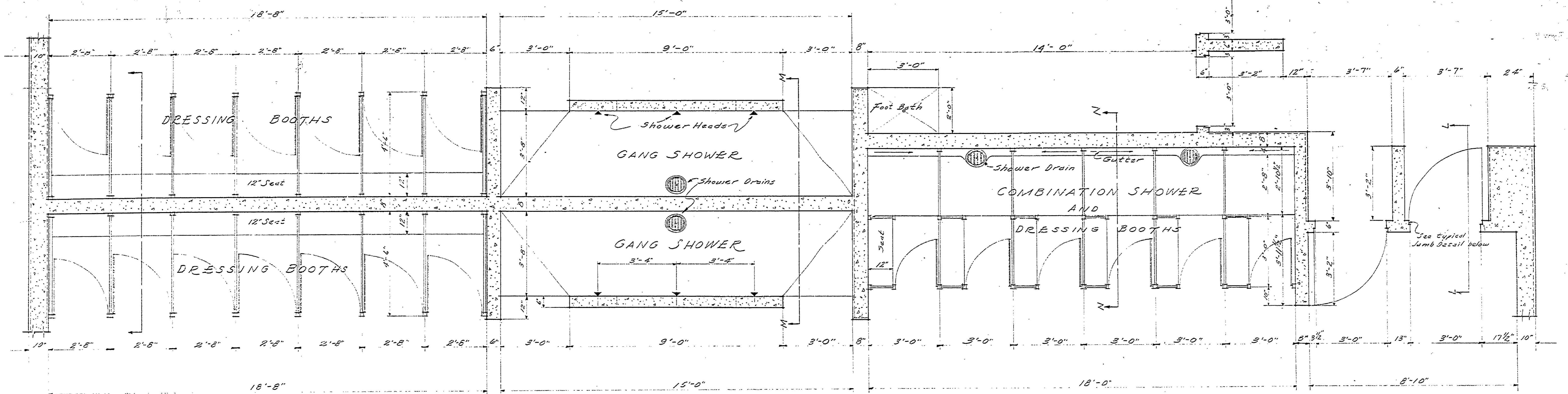
PLAN of SHOWERS & DRESSING BOOTHS Scale 1/2"=1'-0"
