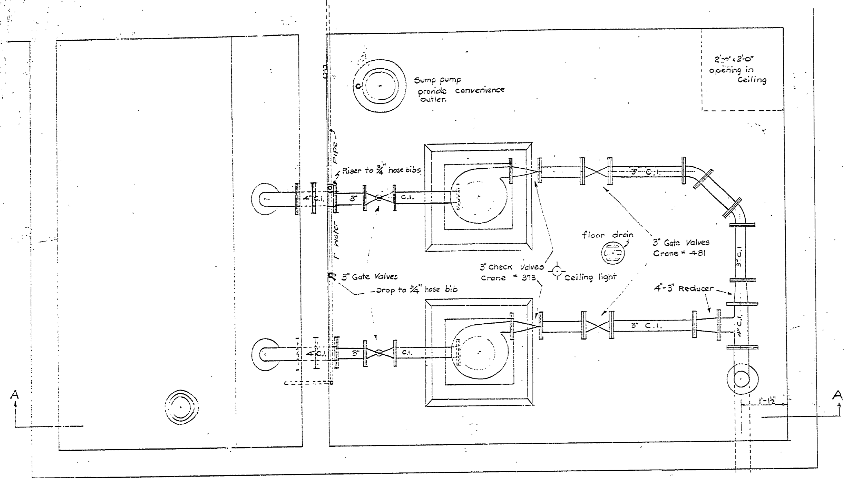
PLAN AT ELEV. 589.00
