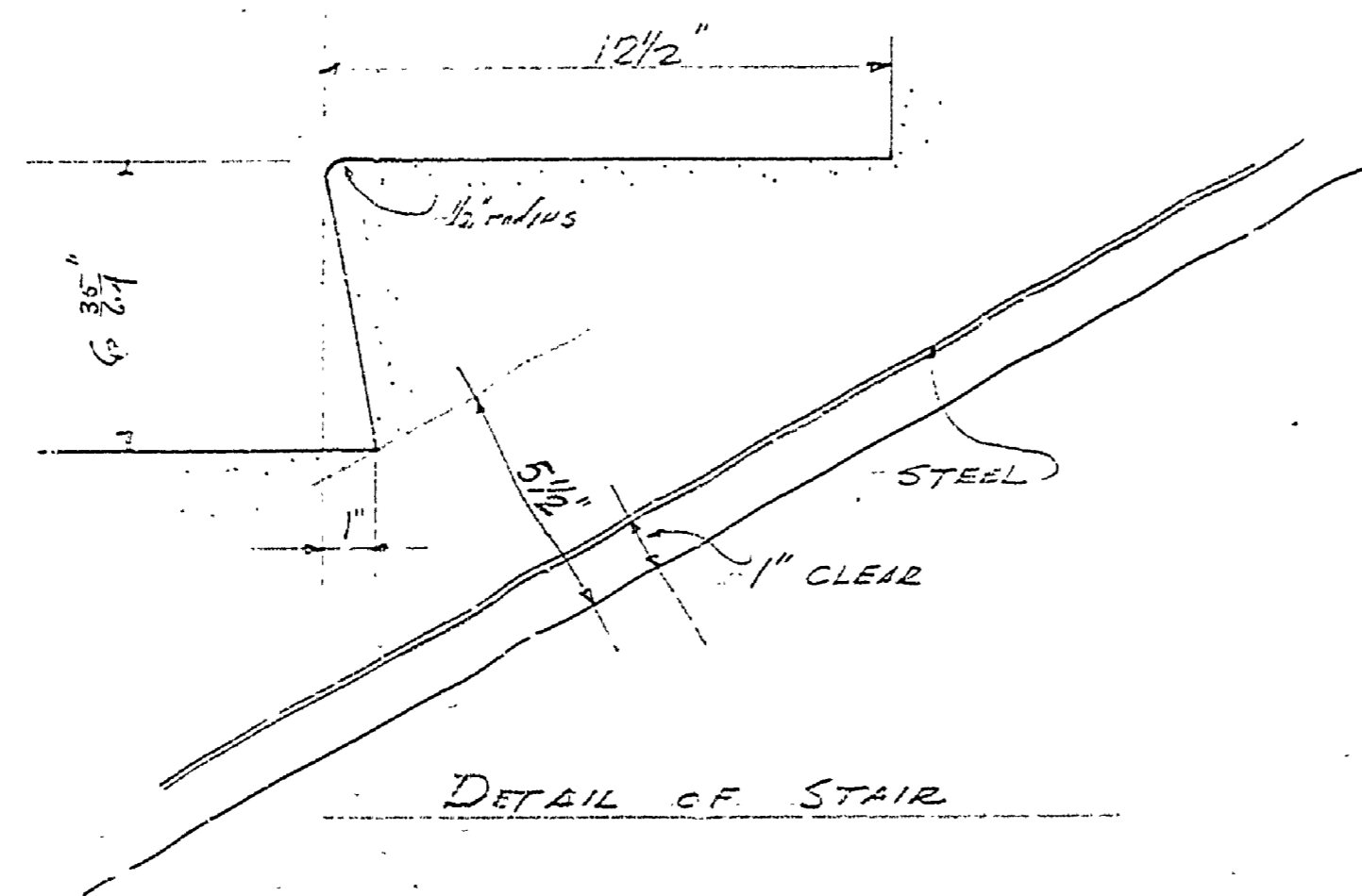
1/2" SCALE SECTION OF STAIR AT SEC. W.W.
