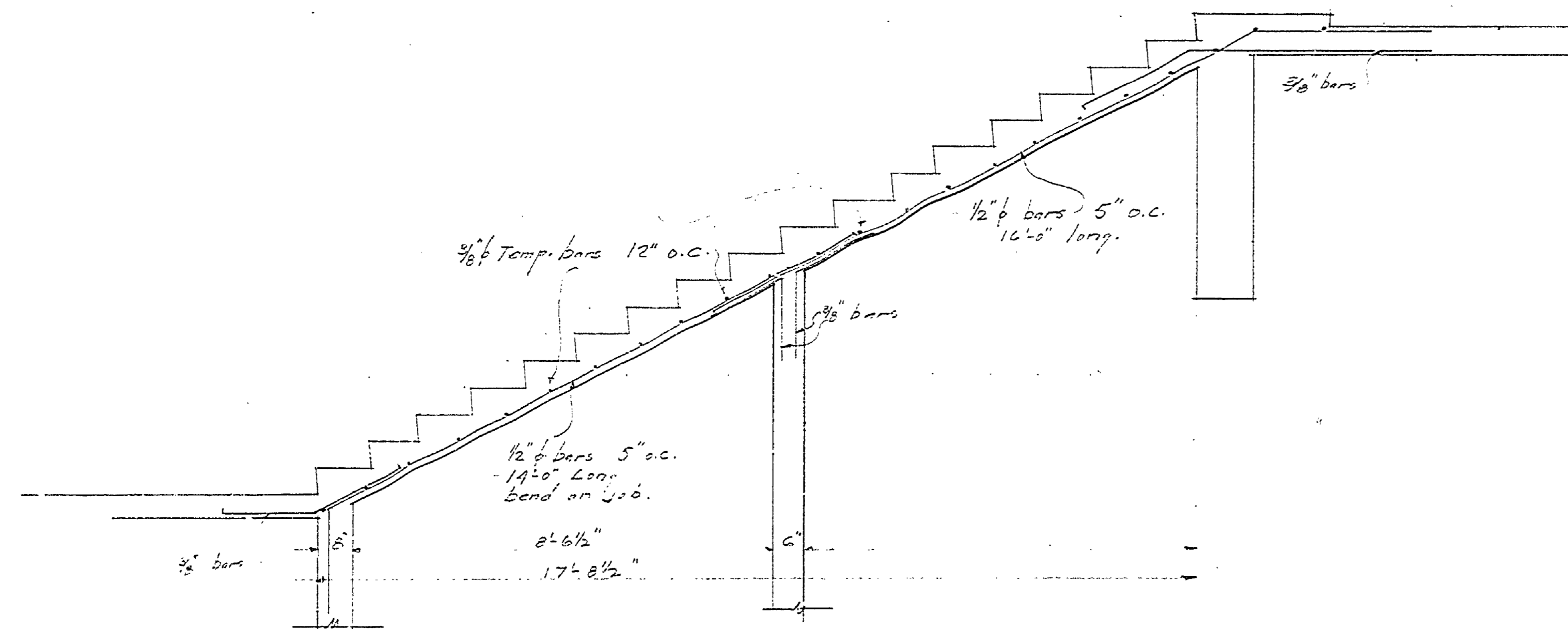
1/2" SCALE SECTION OF STAIR AT SEC. W.W.
