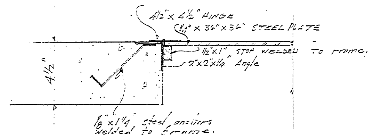
HATCH OPENING 3'-0" x 3'-0" DETAIL OF TRAP DOOR AND FRAME LOCATED AT PUMP ROOM. SCALE 3" = 1'-0"
