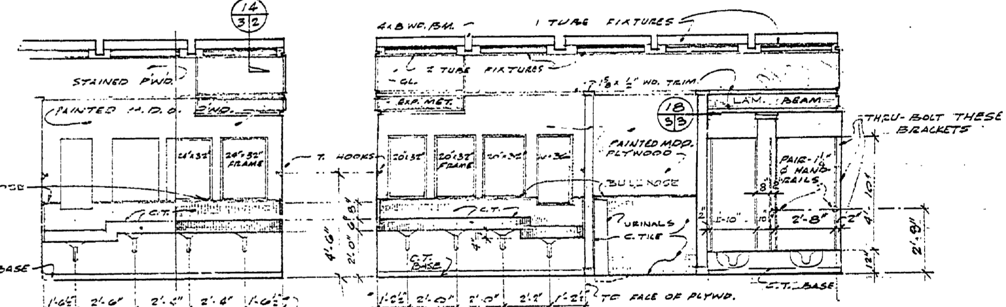
ELEV - WOMEN'S VANITY ELEV - MEN'S TOILET ROOM
