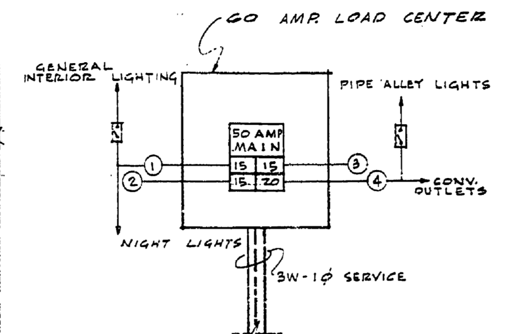
ELECTRICAL SERV.
