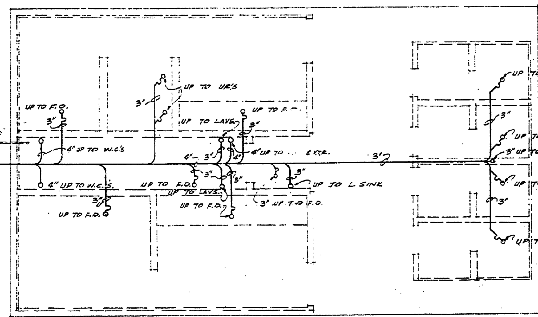
UNDERGROUND PLUMBING
