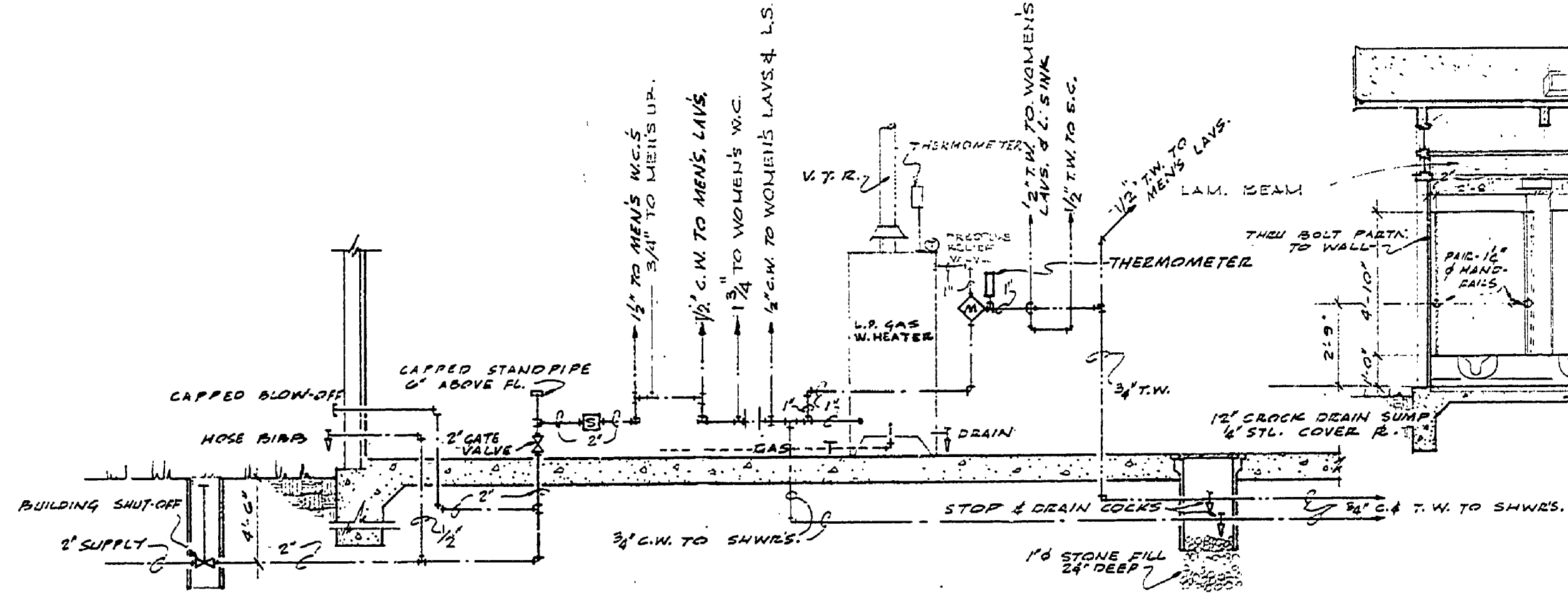
WATER SYSTEM DIAGRAM
