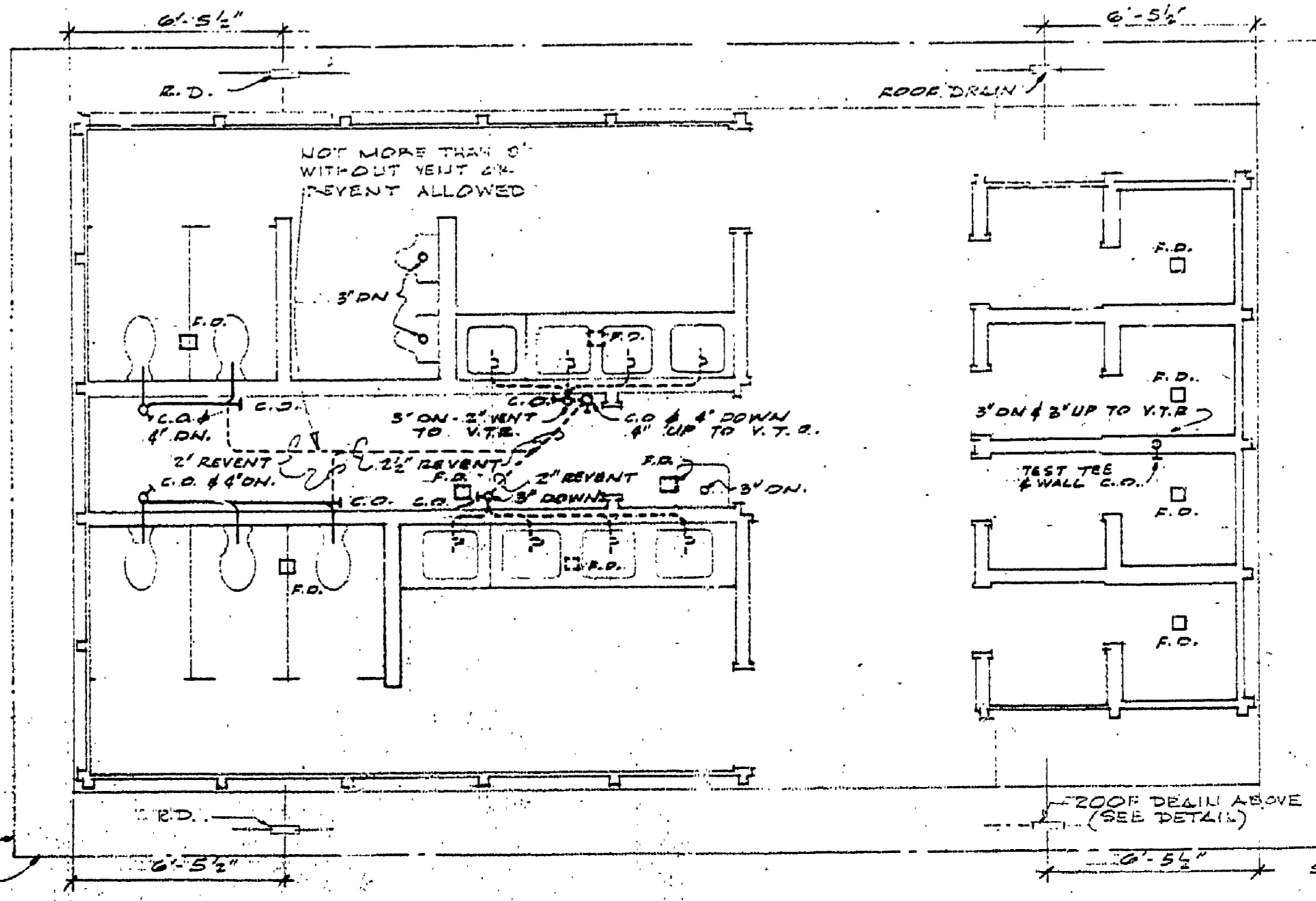
PLUMBING PLAN
