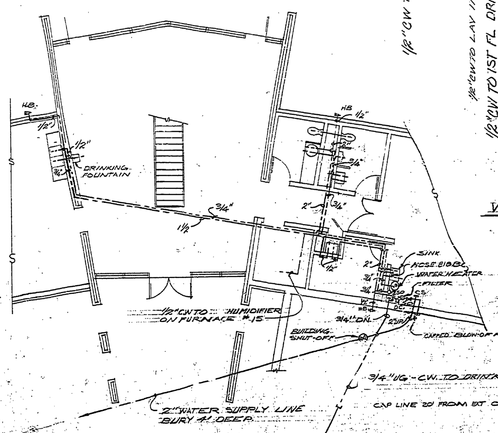
WATER SUPPLY PLAN (FIRST FLOOR) 1/8" = 1'-0"
