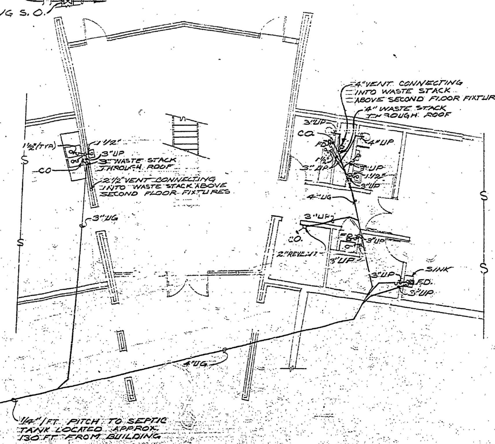
WASTE PLUMBING PLAN (FIRST FLOOR) 1/8" = 1'-0"
