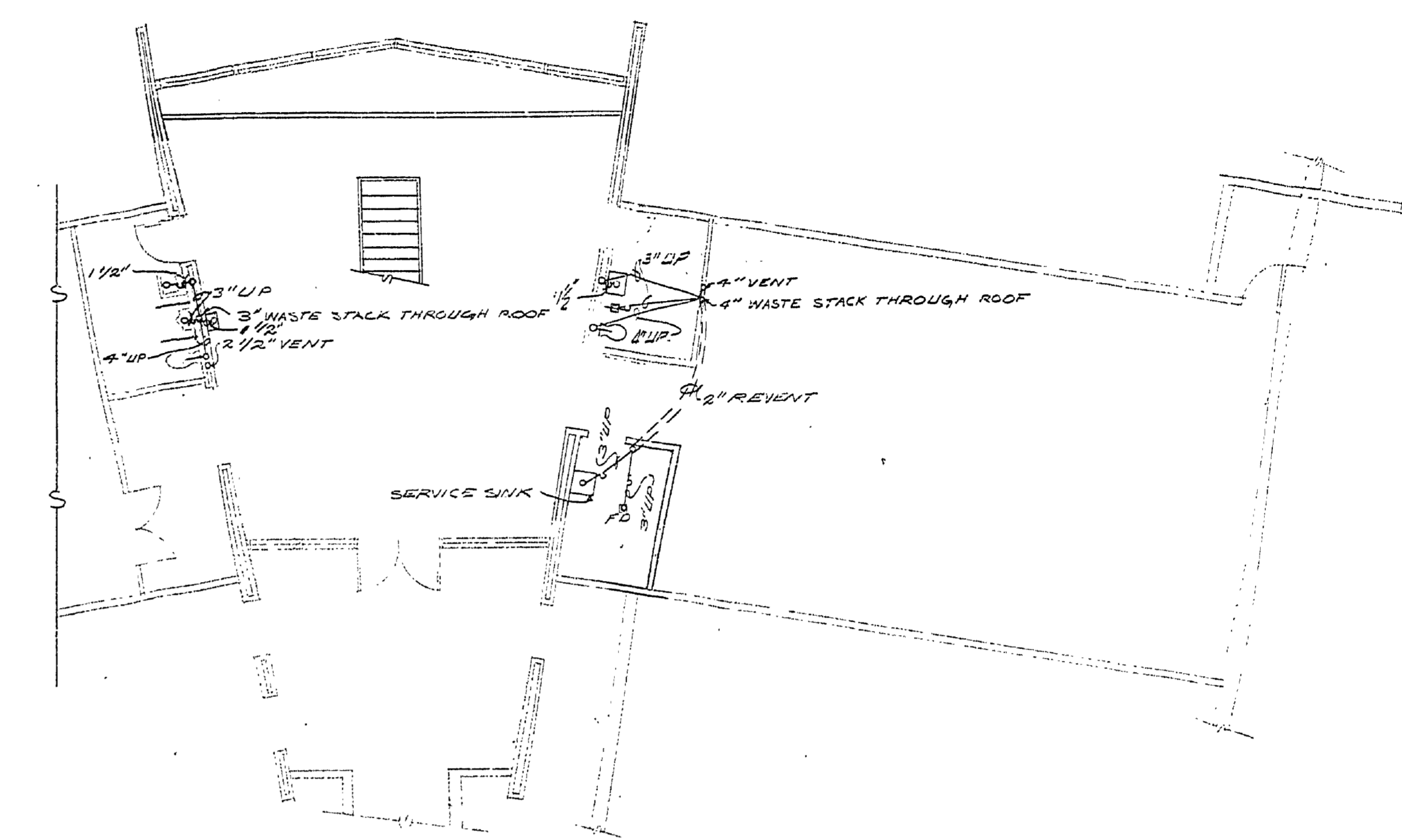
WASTE PLUMBING PLAN (SECOND FLOOR) 1/8" = 1'-0"
