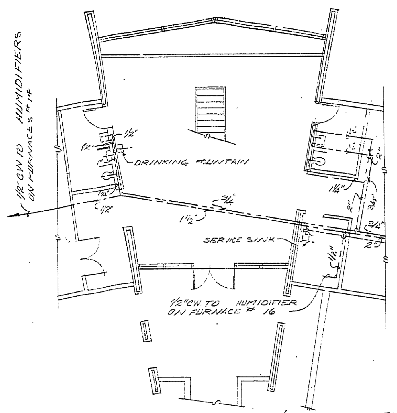
WATER SUPPLY PLAN (SECOND FLOOR) 1/8" = 1'-0"
