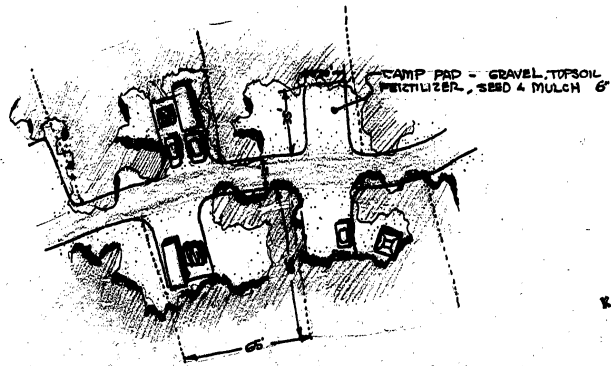
TYPICAL CAMPSITE LAYOUT SCALE 1" = 30'
