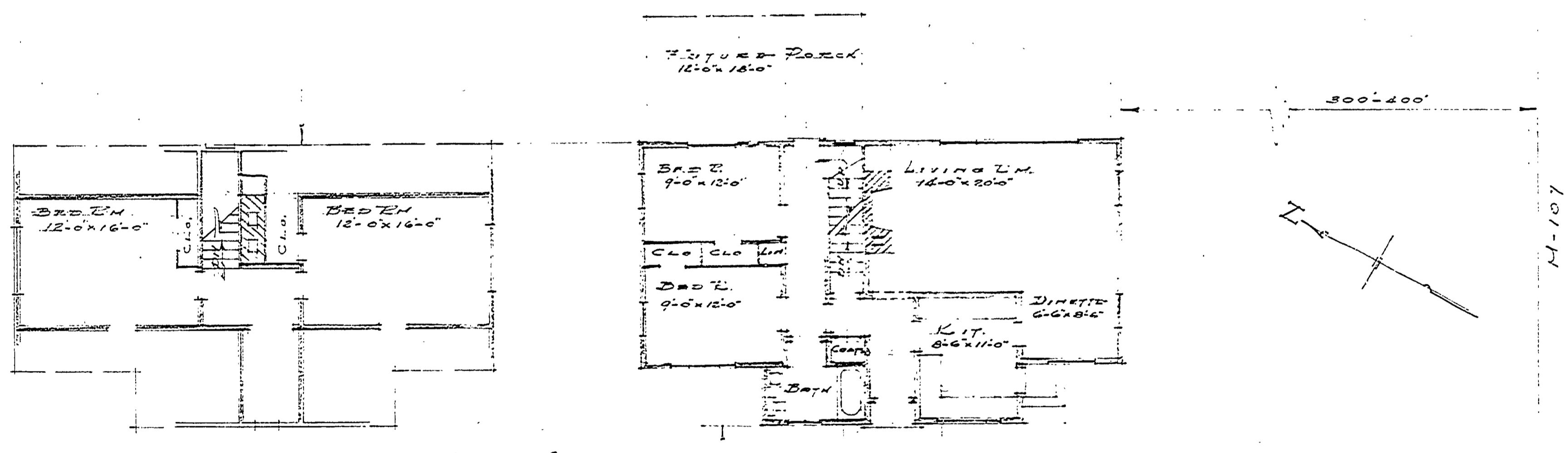
SECOND FLOOR PLAN Scale 1/4" = 1'-0"
