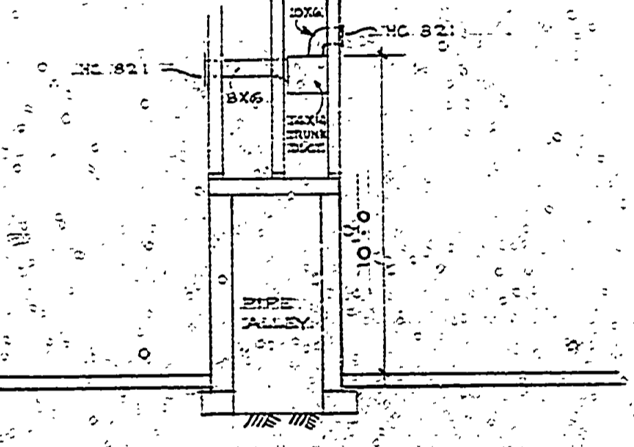
SECTION SHOWING TRUNK DUCT AND SUPPLY DUCTS ABOVE PIPE ALLEY. 1/4" = 1'-0"
