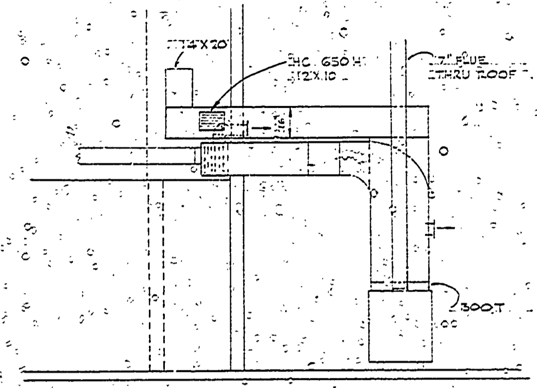
ELEVATION OF FURNACE SHOWING CONNECTION TO TRUNK DUCT. RETURN AIR GRILLE ABOVE AND FEEDER DUCT TO LAUNDRY ROOM. 1/4" = 1'-0"
