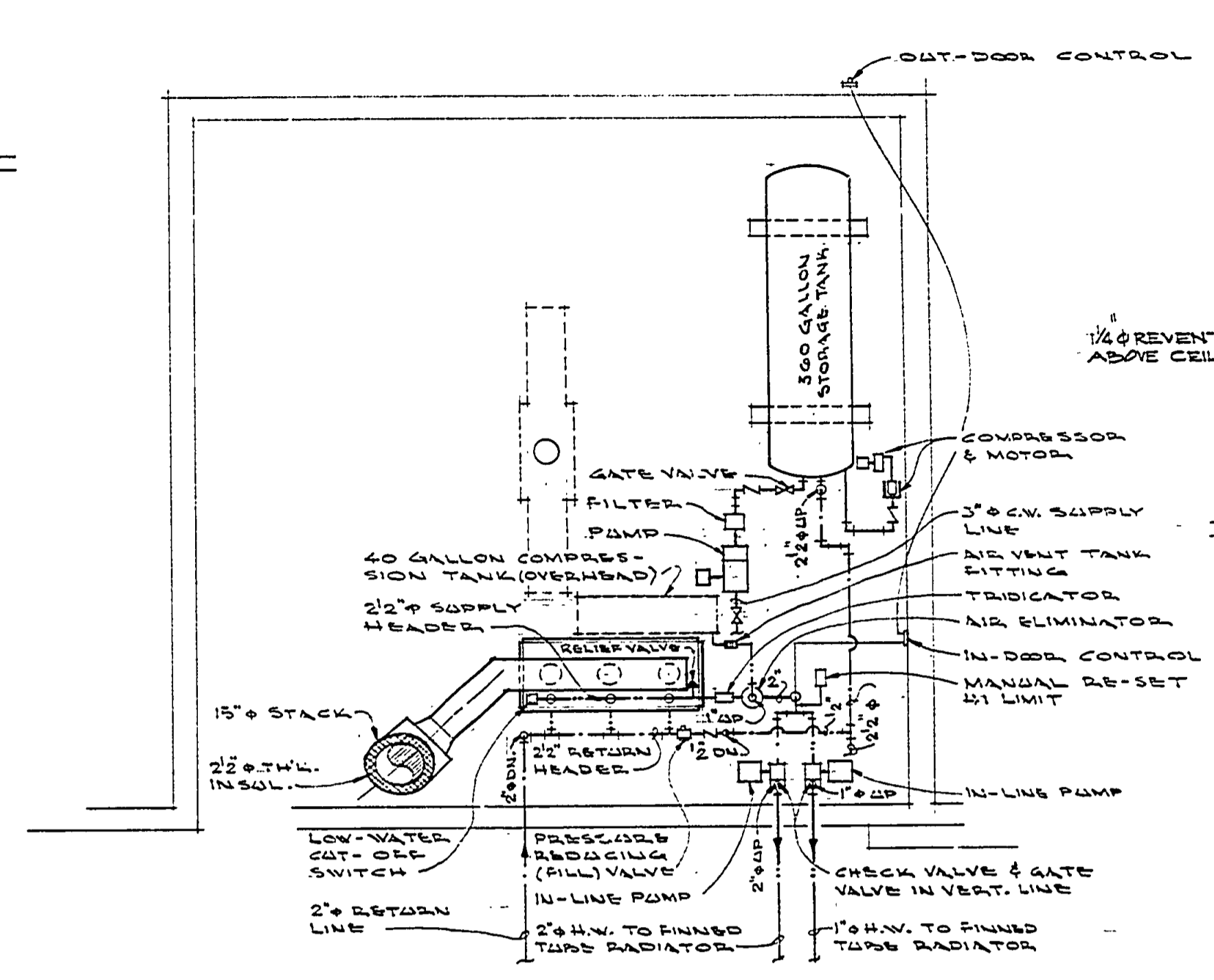
PLAN - BASEMENT BOILER ROOM WATER SUPPLY PLUMBING SC. 1/2" = 1'-0"
