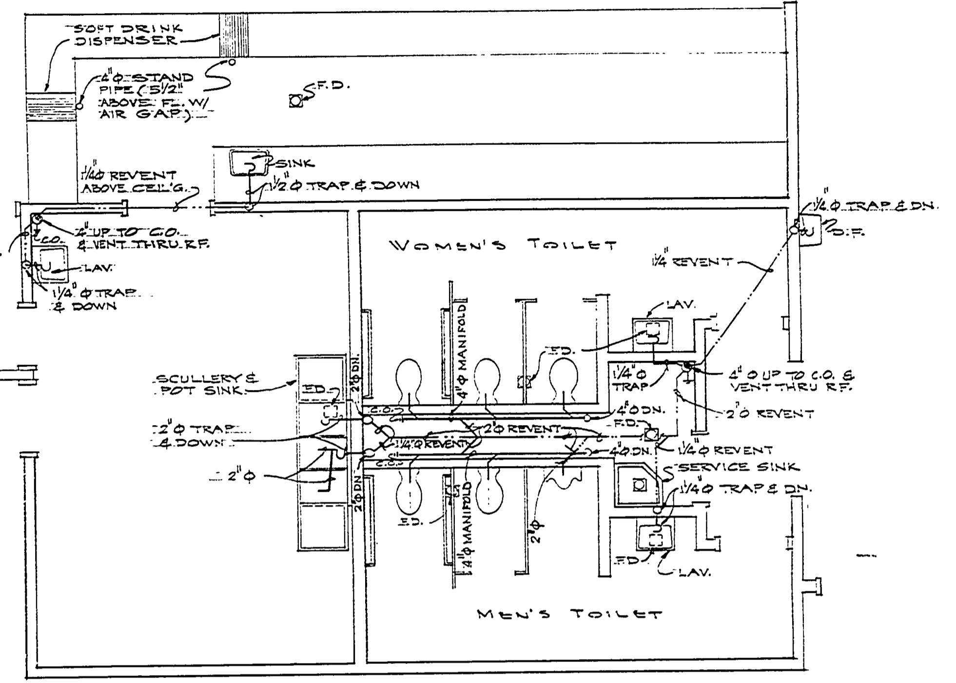
PLAN - FIRST FLOOR WASTE PLUMBING SC. 1/2" = 1'-0"
