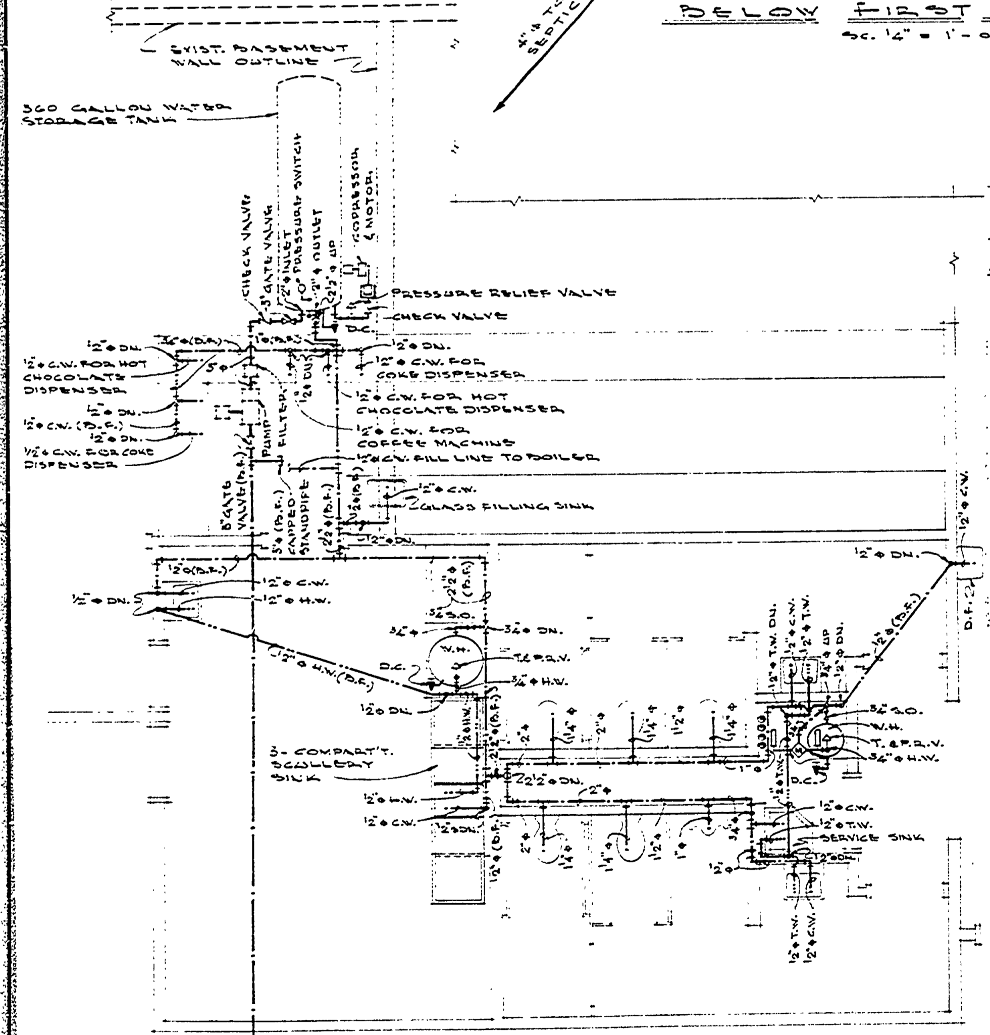
PLAN - BASEMENT & FIRST FLOOR WATER SUPPLY PLUMBING SC. 1/2" = 1'-0"
