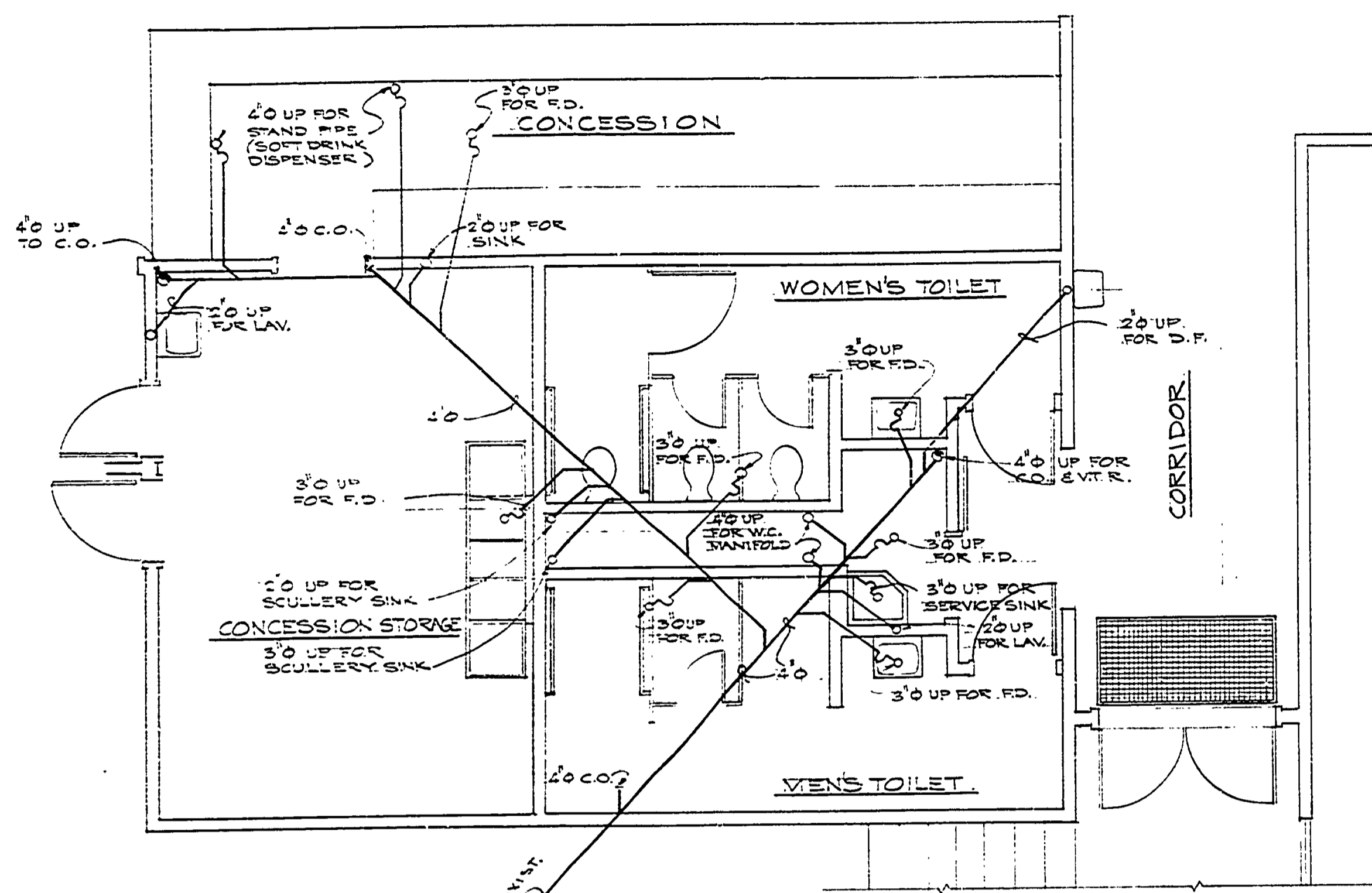
PLAN - WASTE PLUMBING DETAIL FIRST FLOOR SC. 1/2" = 1'-0"
