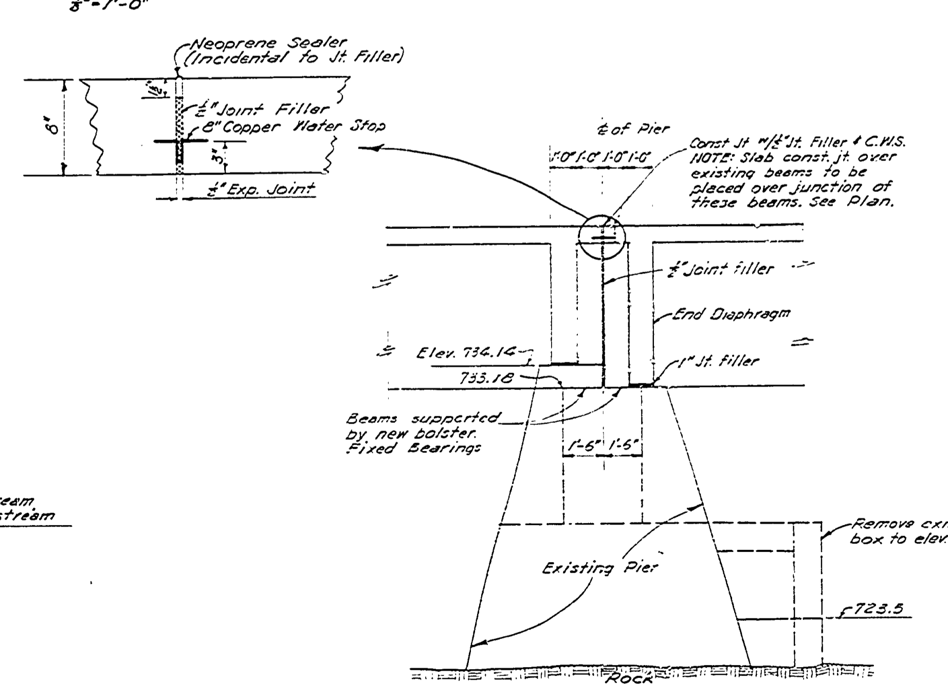
SECTION B-B 1/4"=1'-0"
