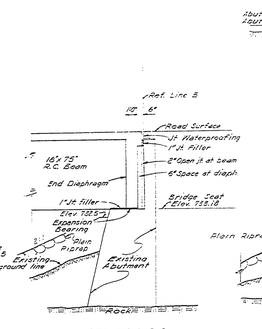
SECTION C-C 1/4"=1'-0"
