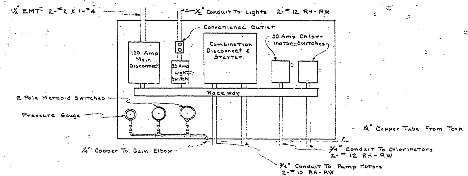
PANELBOARD DETAIL Not To Scale
