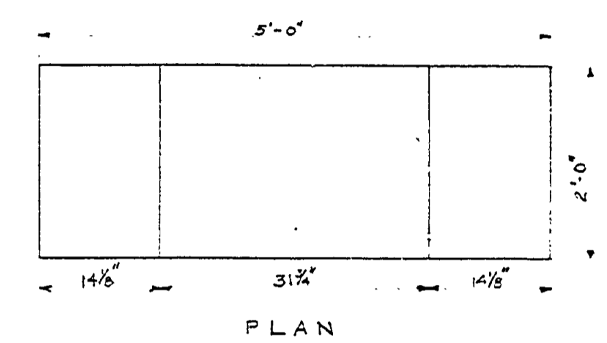
PLAN SECTION TANK SUPPORT DETAIL
