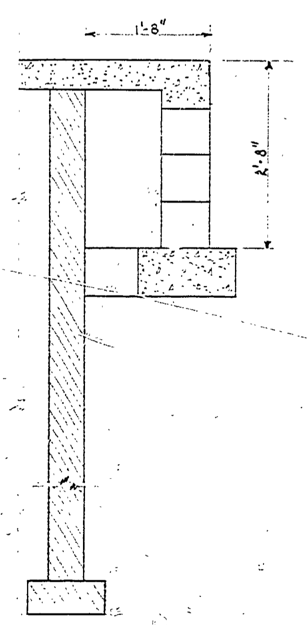
SECTION C-C
