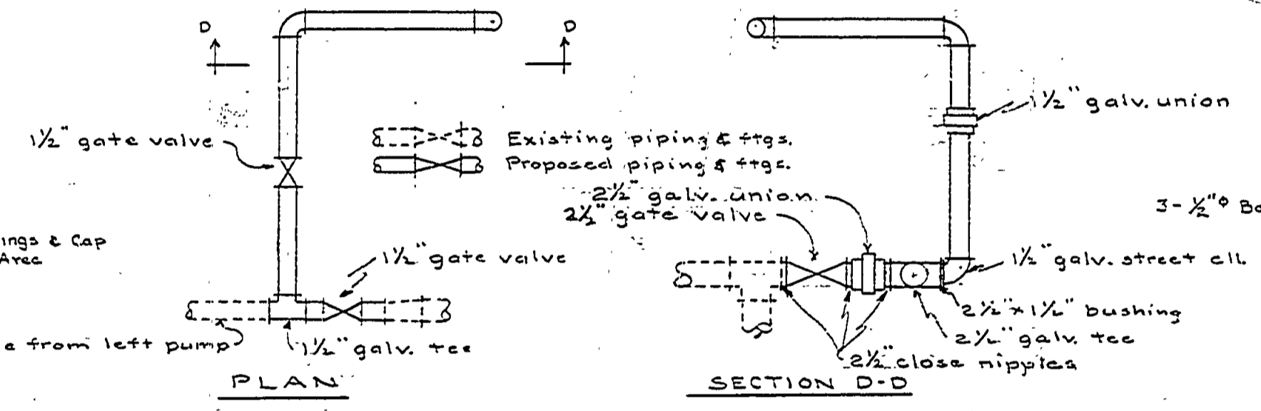
DETAIL FOR CONNECTING PUMPS TO OPERATE IN SERIES OR ALTERNATELY
