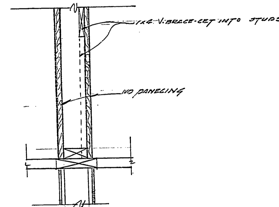
SECT. 2-2
