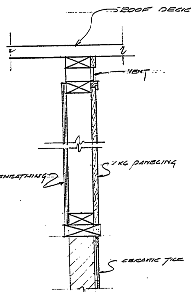
SECT. 1-1
