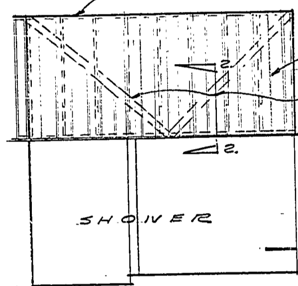
ELEVATION @ SHOWER SHOWING WALL BRACING
