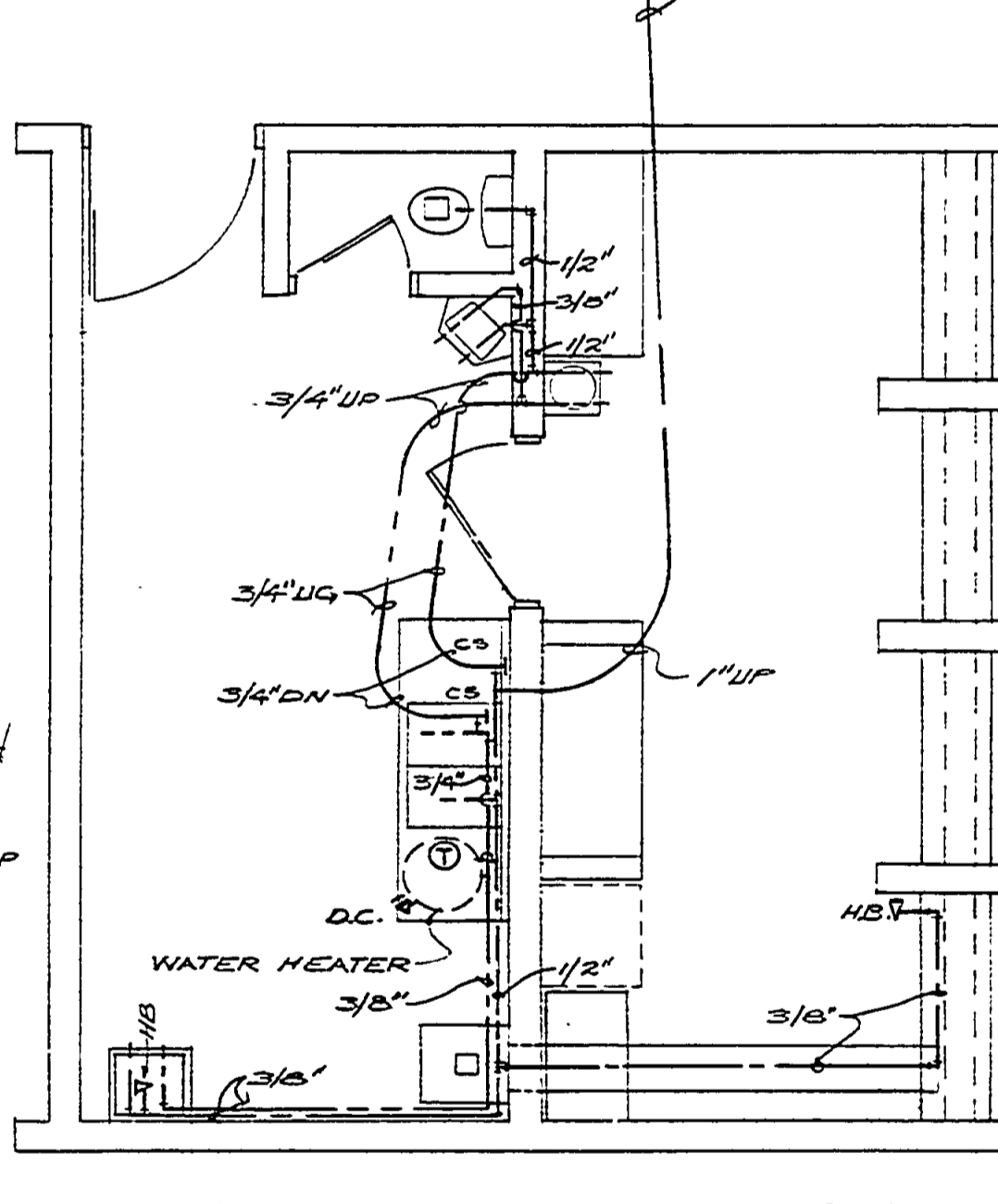
SUPPLY PLUMBING PLAN
