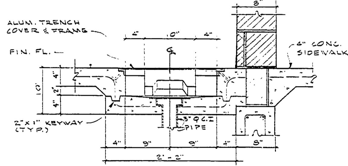
DETAIL 32 S.C. 1/2" = 1'-0"
