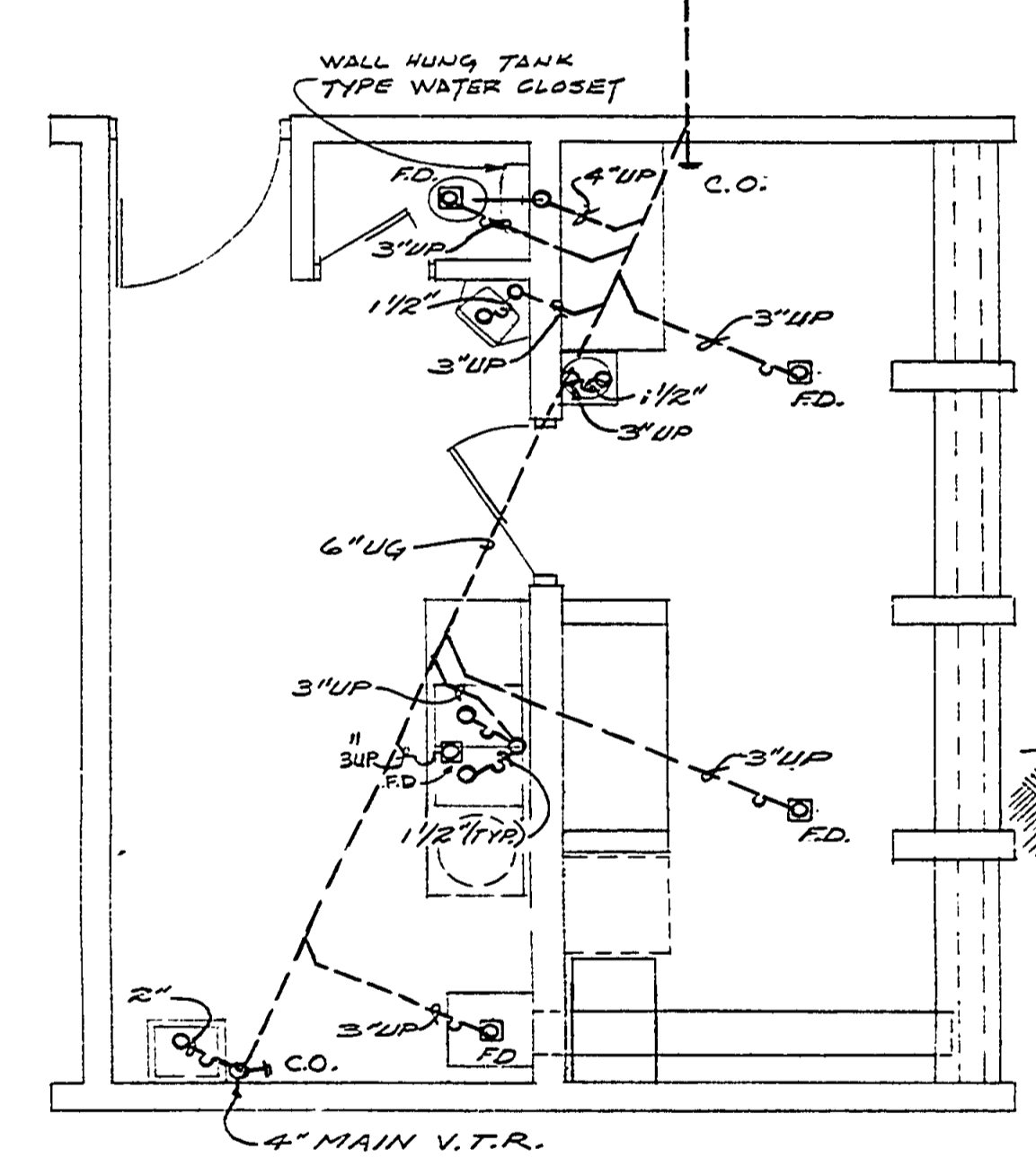
WASTE PLUMBING PLAN 1/4" = 1'-0"
