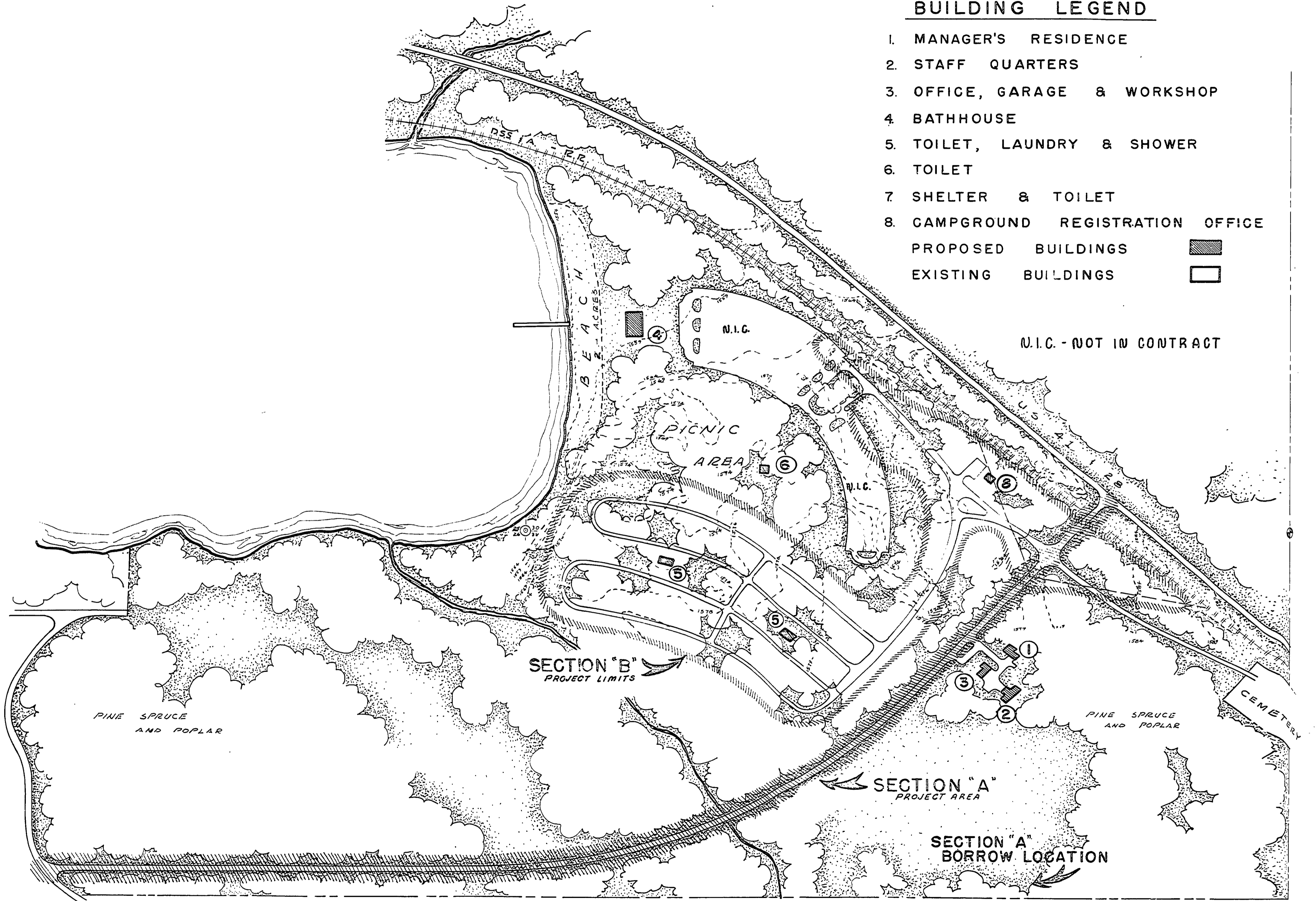
SITE DEVELOPMENT PLAN SCALE 1" = 200' 0"
