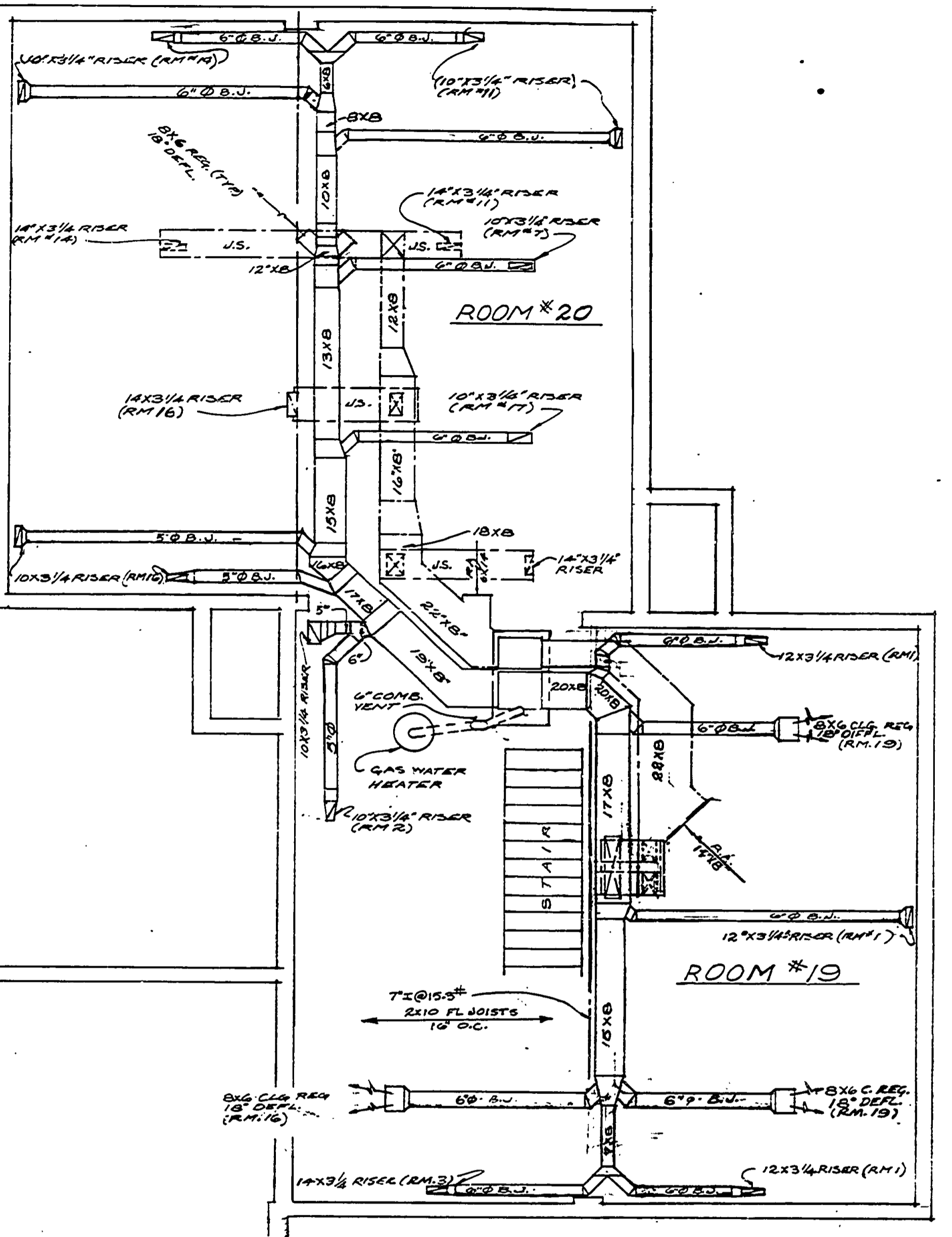
HEATING PLAN - BASEMENT SCALE: 1/8" = 1'-0"
