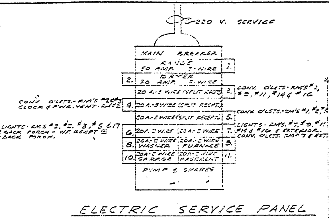
ELECTRIC SERVICE PANEL
