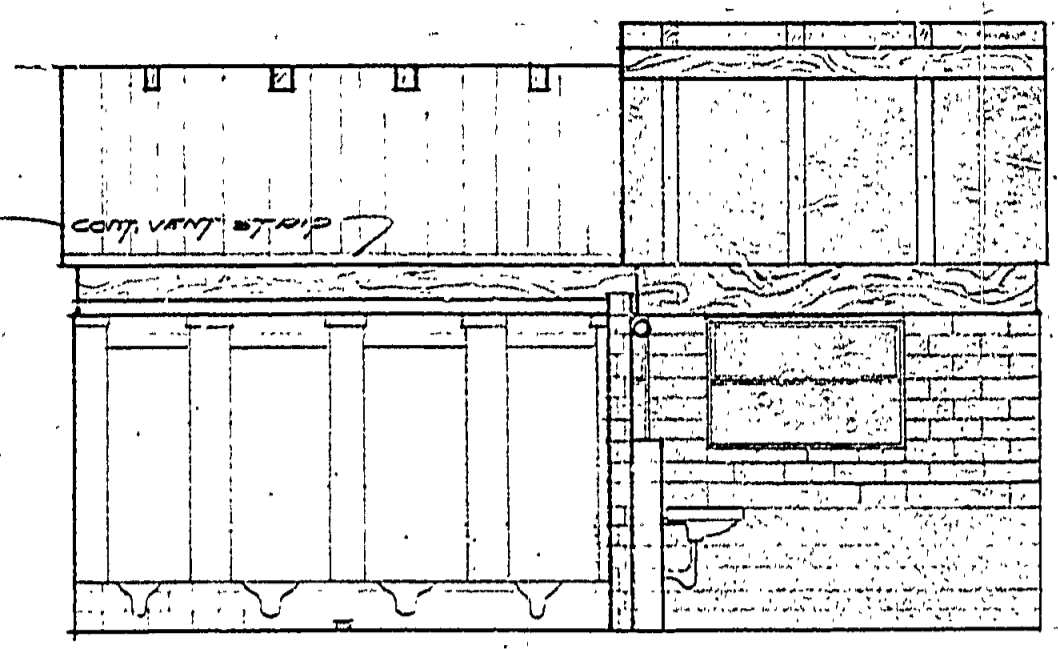
INT. ELEV. WEST WOMEN'S TOILET SCALE 1/4"=1'-0"
