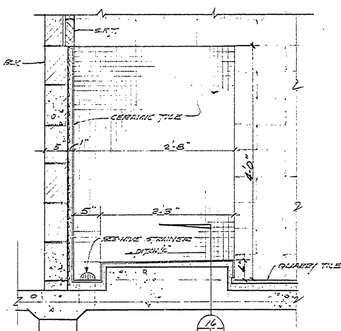
WATER HEATER PIPING
