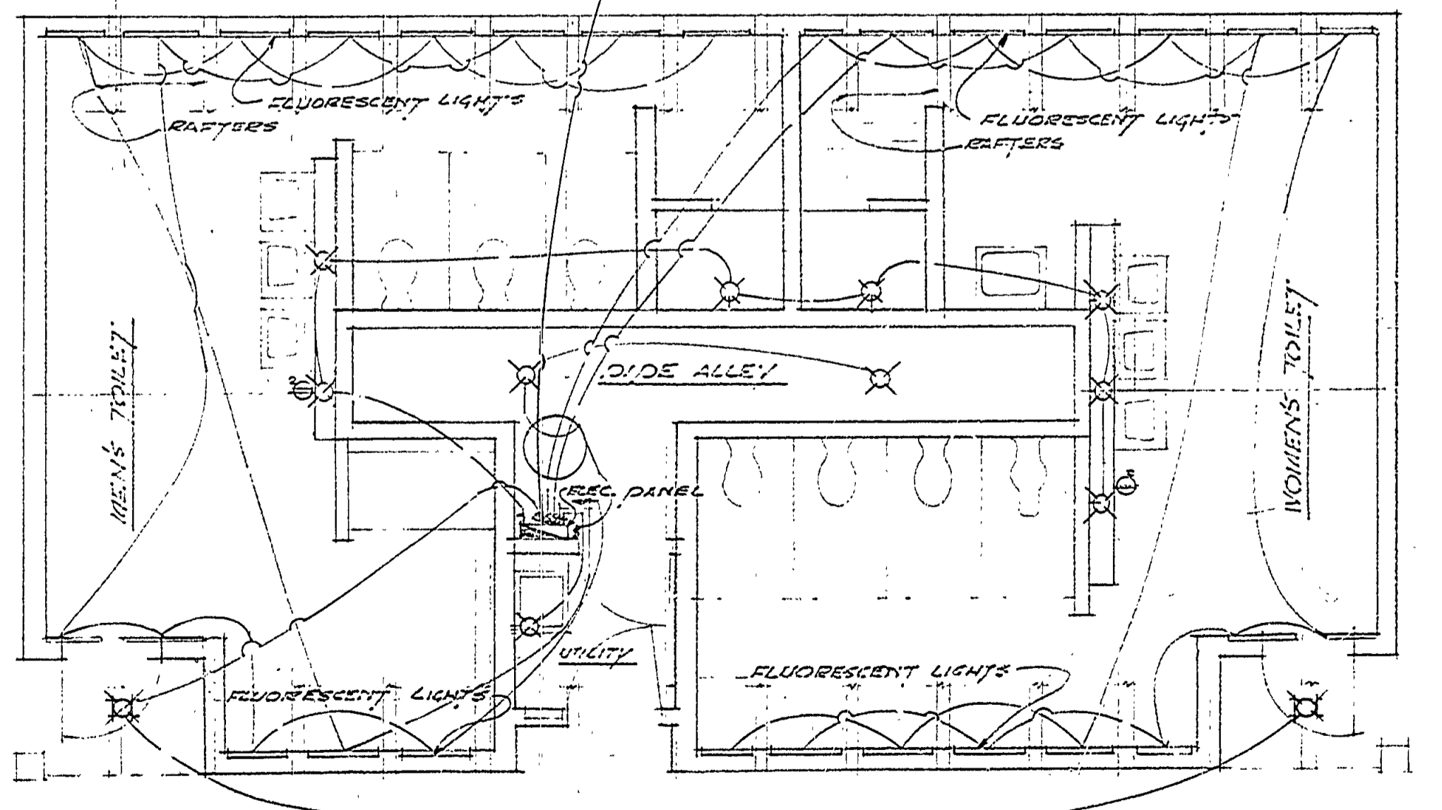
ELECTRICAL PLAN SCALE 1/4"=1'-0"
