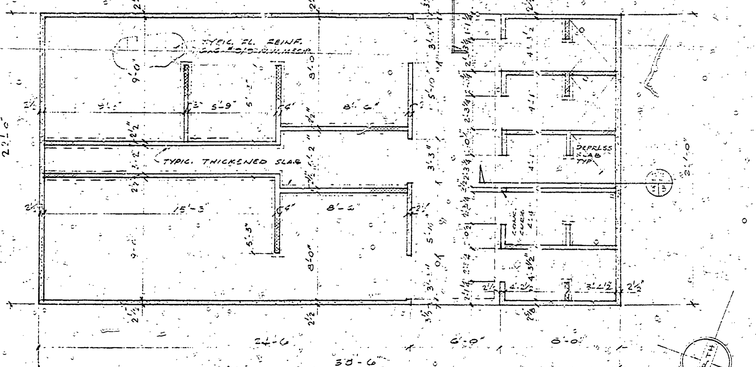
FOUNDATION PLAN
