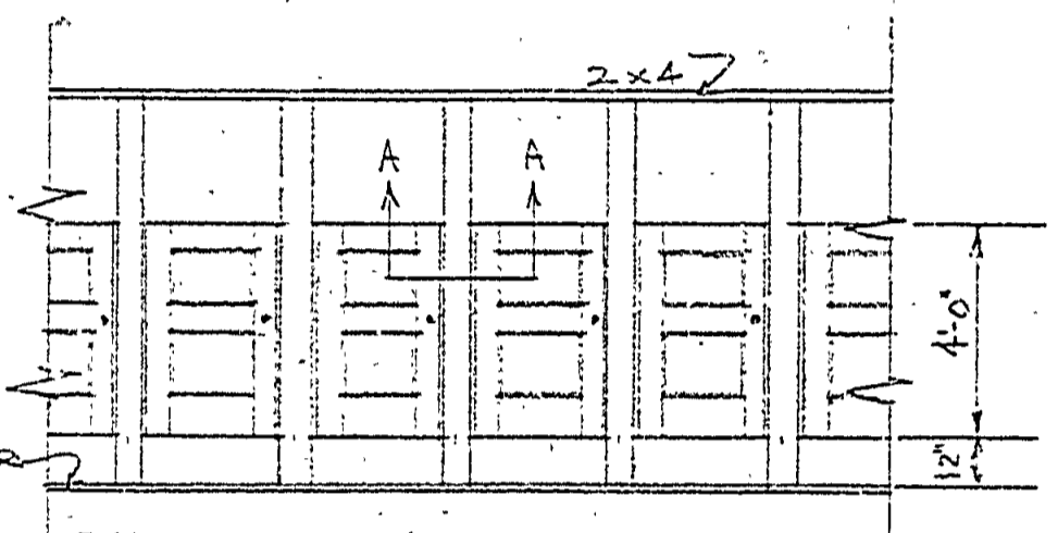
TYPICAL ELEVATION BOOTHS SCALE 1/2" = 1 FT.
