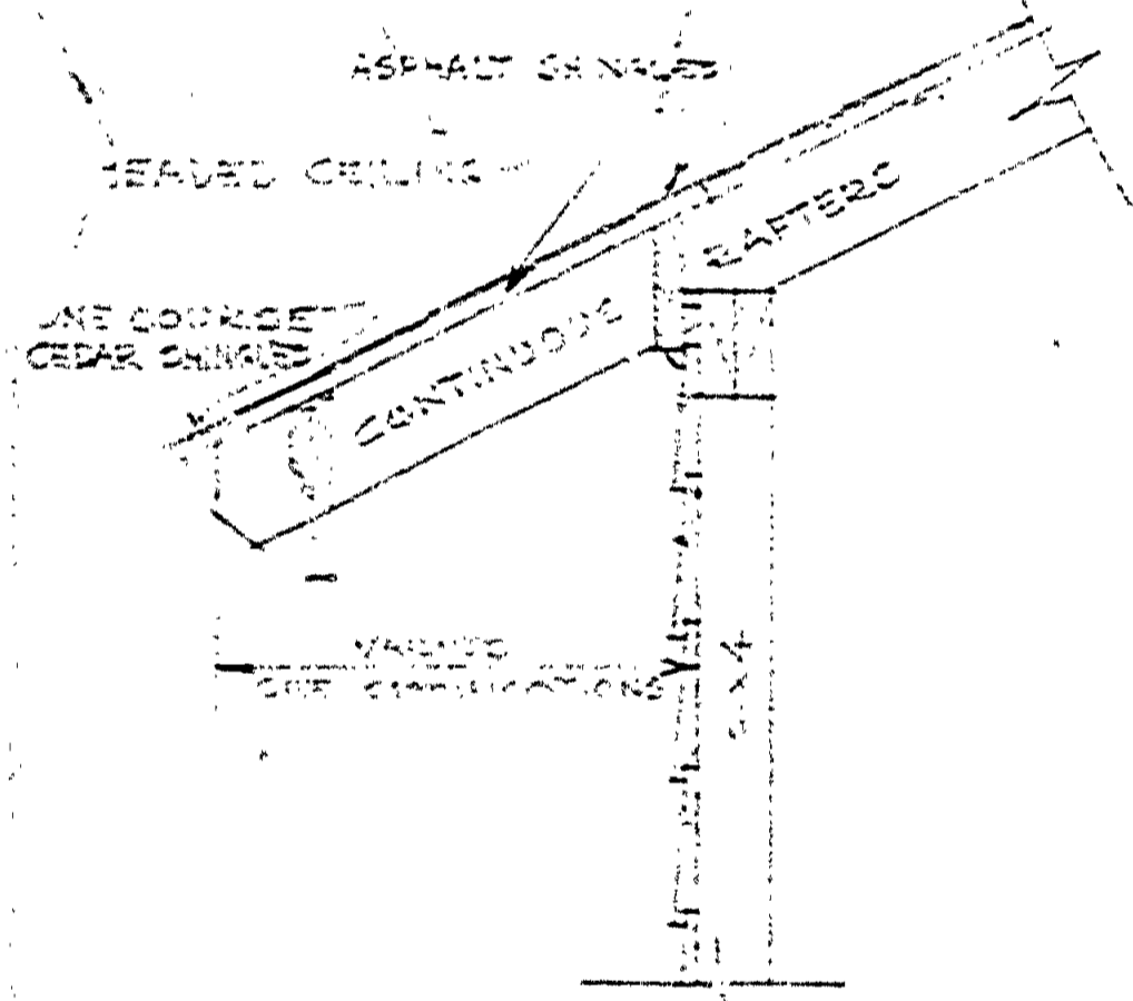
TYPICAL DETAIL AT EAVES SCALE 1" = 1 FT.
