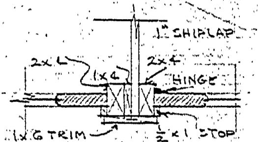
TYPICAL WINDOW HEAD & SILL DETAIL SCALE 1" = 1 FT.
