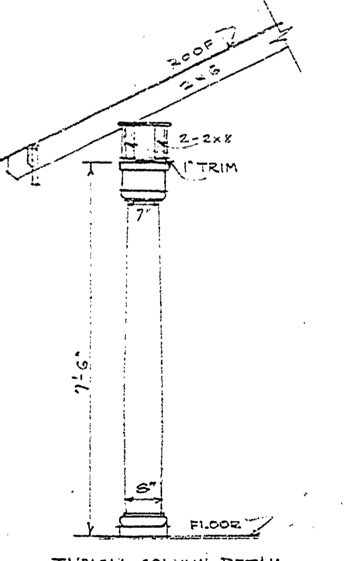
TYPICAL COLUMN DETAIL 6 REQUIRED FULL ROUND 2 REQUIRED HALF ROUND SCALE 1/2" = 1 FT.
