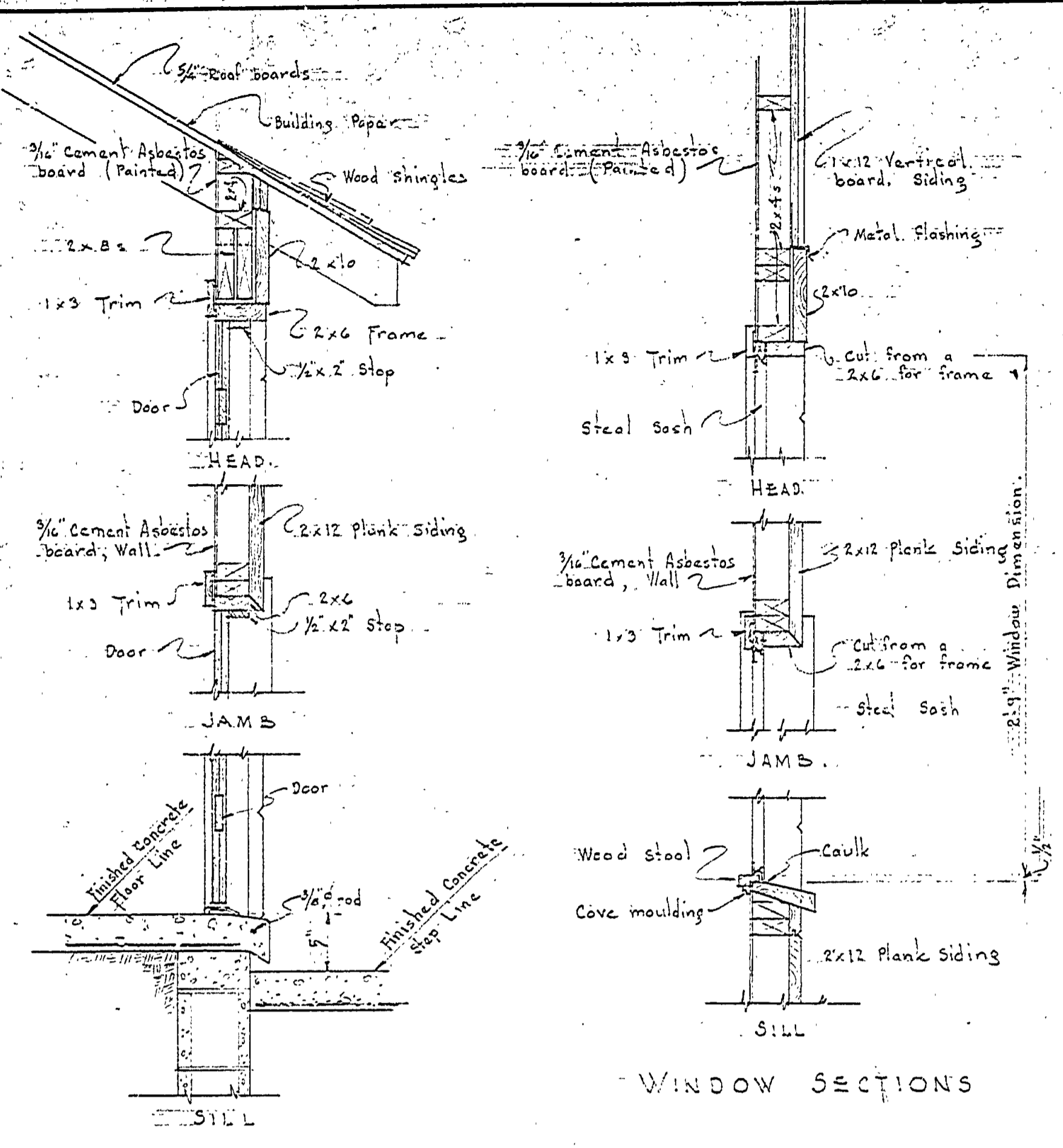
TYPICAL DETAILS LAUNDRY AND STORAGE ROOM Scale 1/4" = 1'-0"
