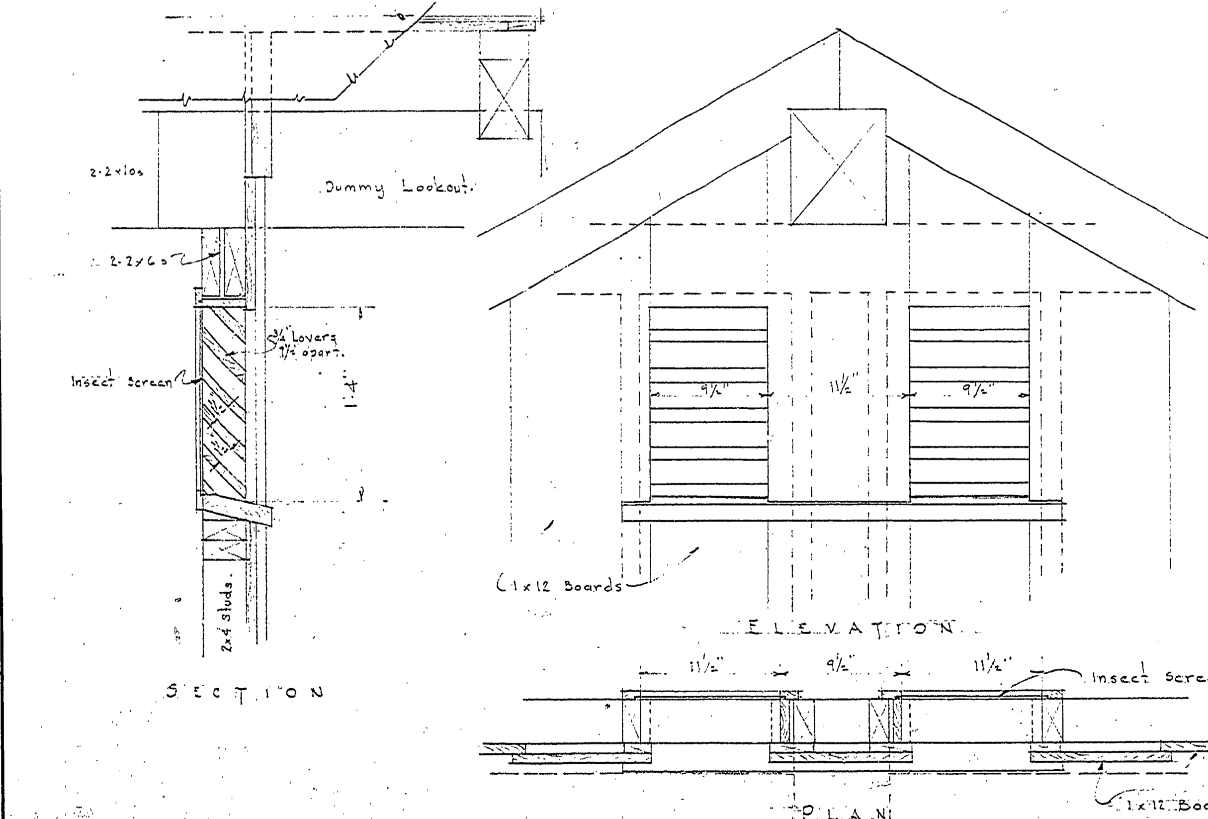
LOUVER DETAIL Scale 1/4" = 1'-0"
