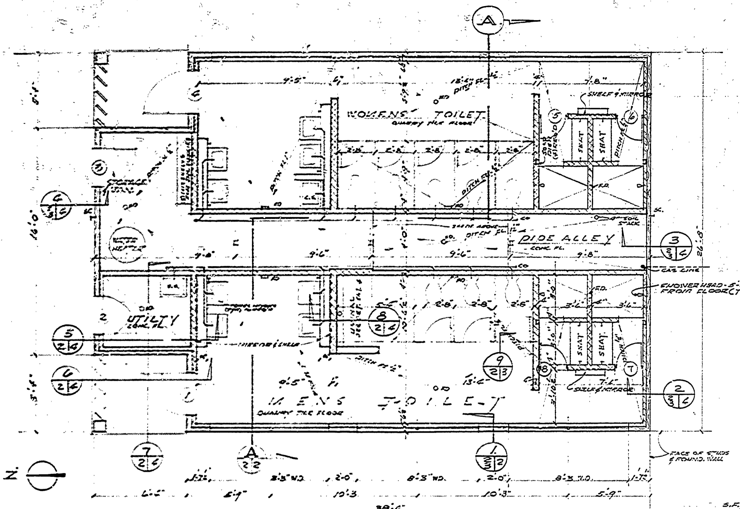
FLOOR PLAN Scale 1/4\"/>
