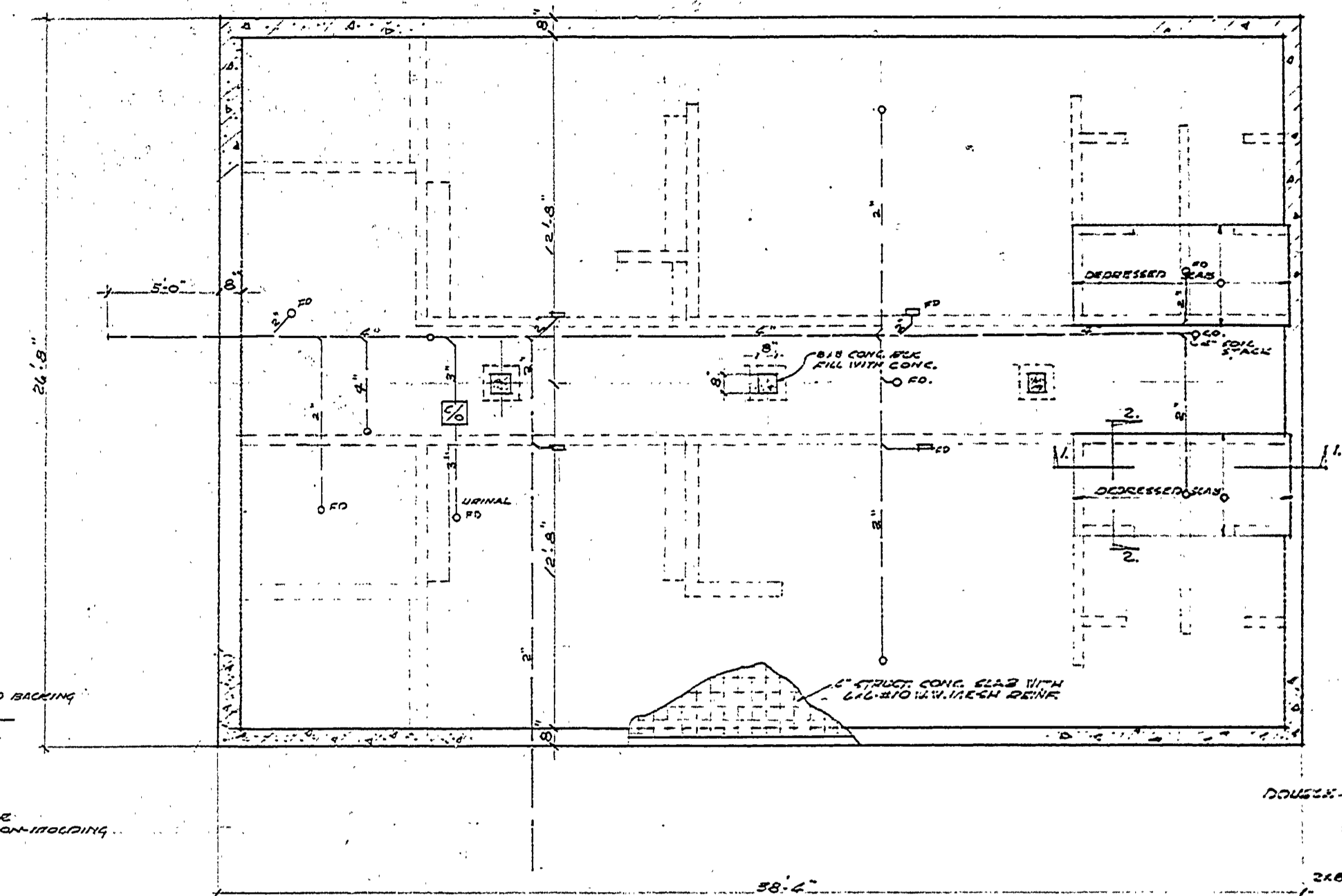
FOUNDATION AND PLUMBING PLAN Scale 1/4\"/>
