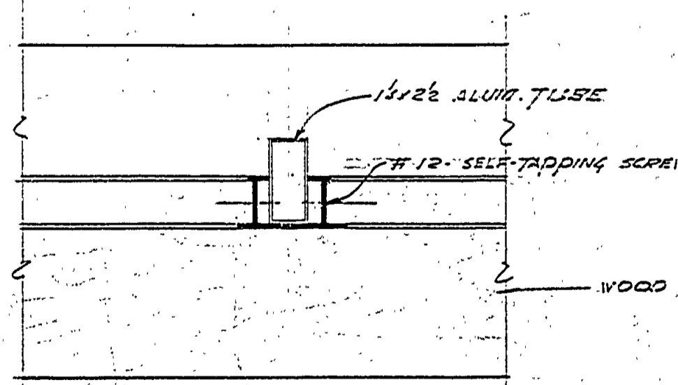
MULLION DET Scale 5/16\"/>
