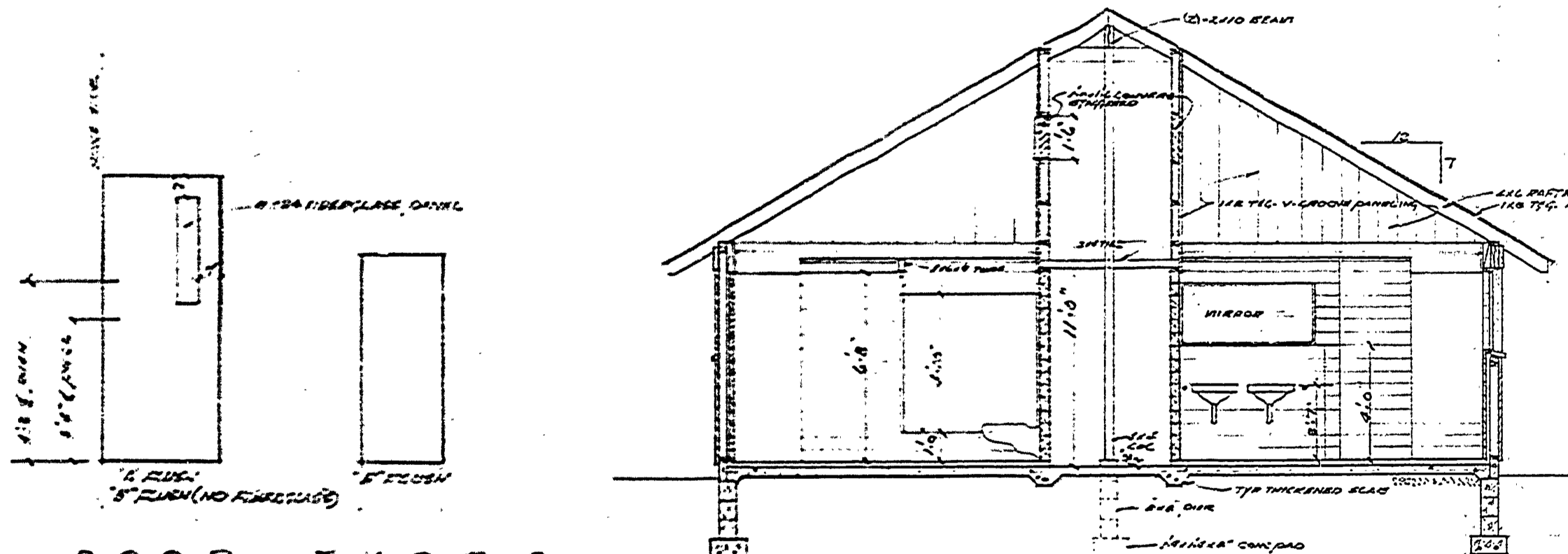
SECTION AA
