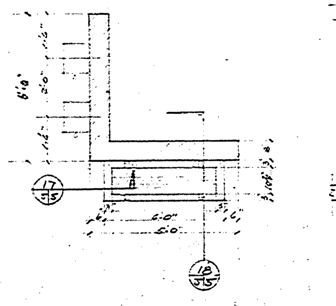
PLAN SECTION-WATER STATION
