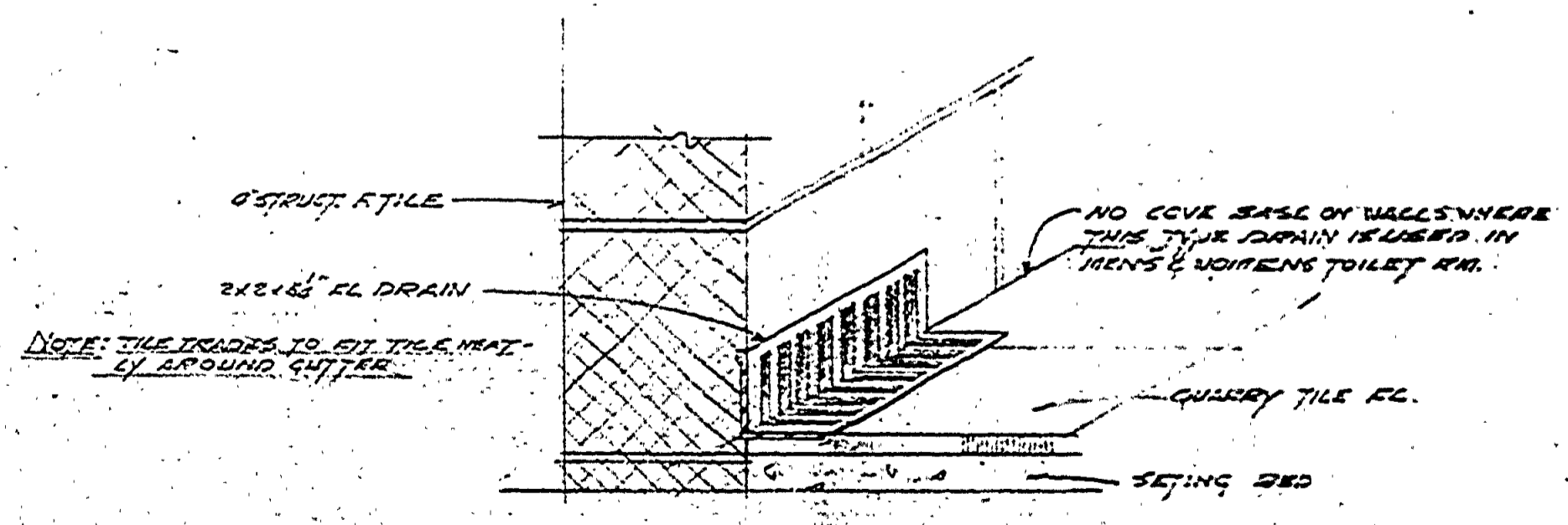
DET. OF GUTTER TYPE FL. DRAIN (REV'D)
