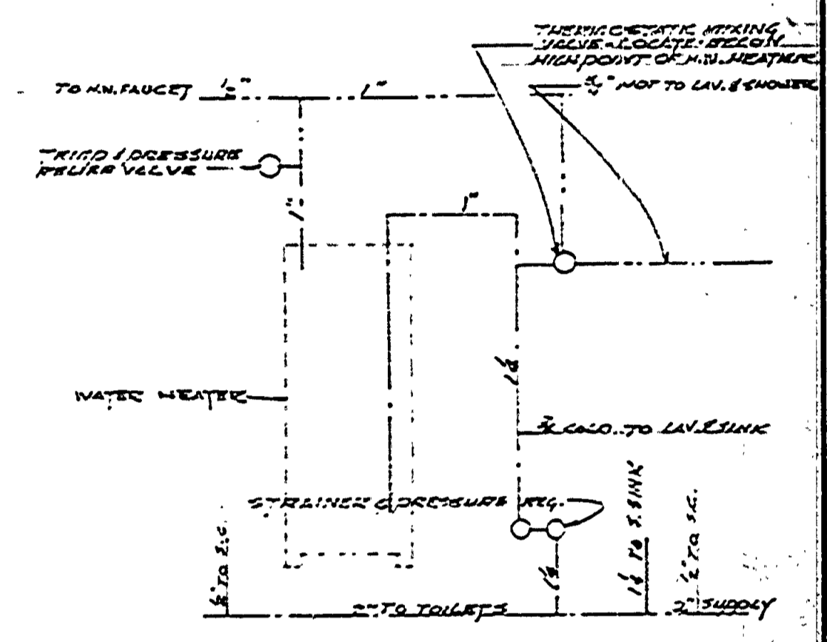
HOT WATER PIPING
