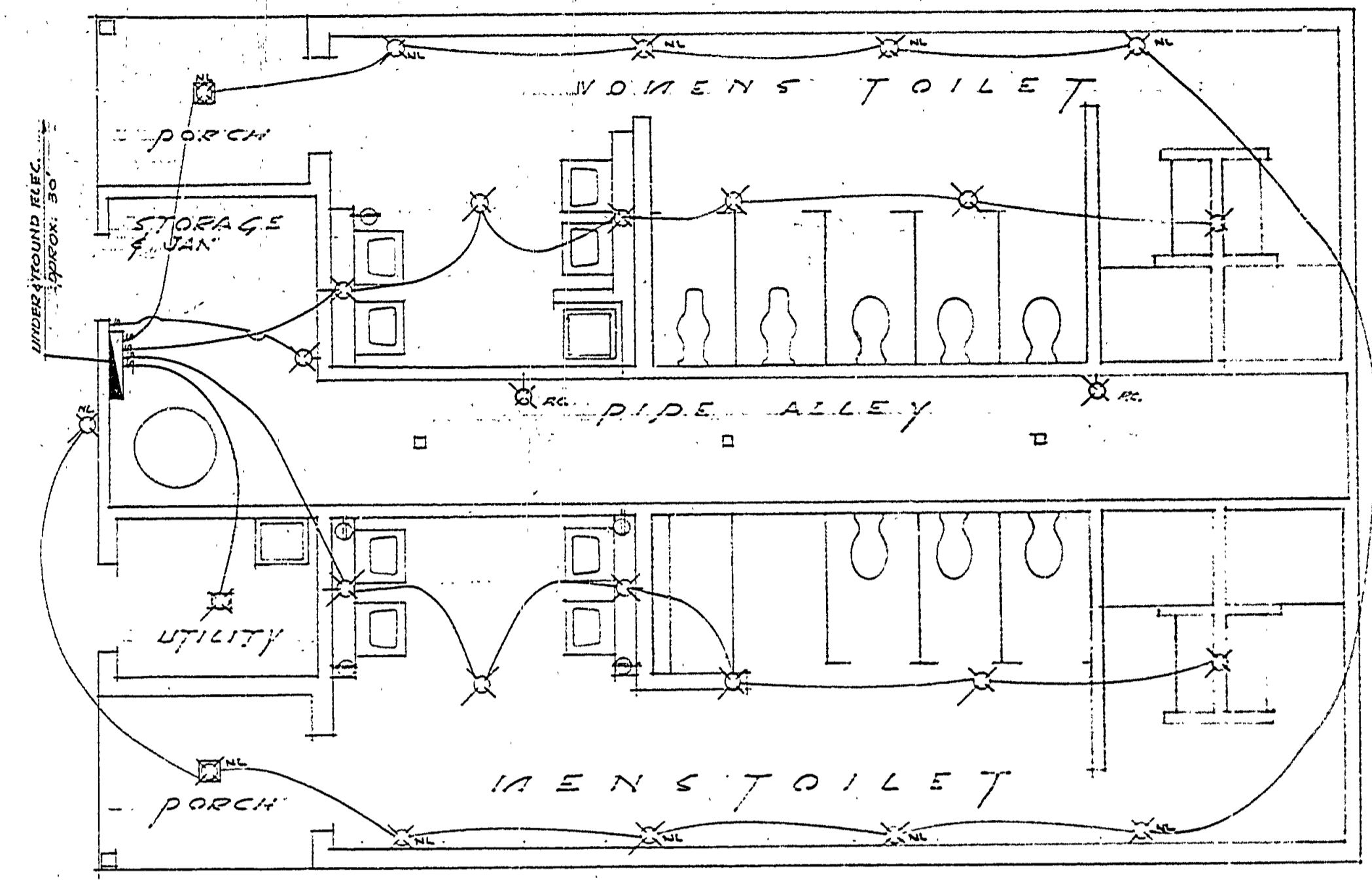
ELECTRICAL PLAN
