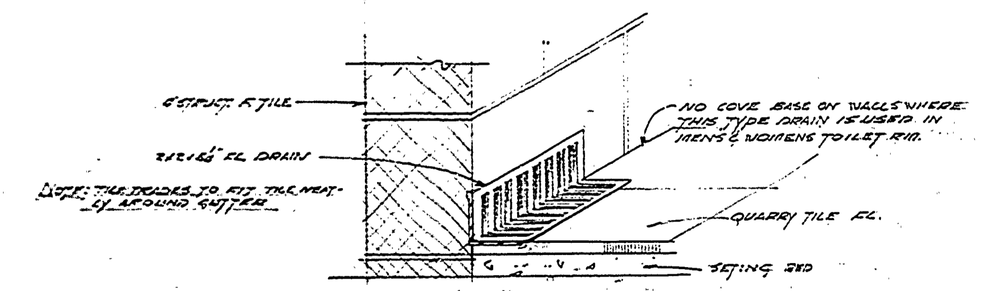
DET. OF GUTTER TYPE FL. DRAIN (AREA 10)
