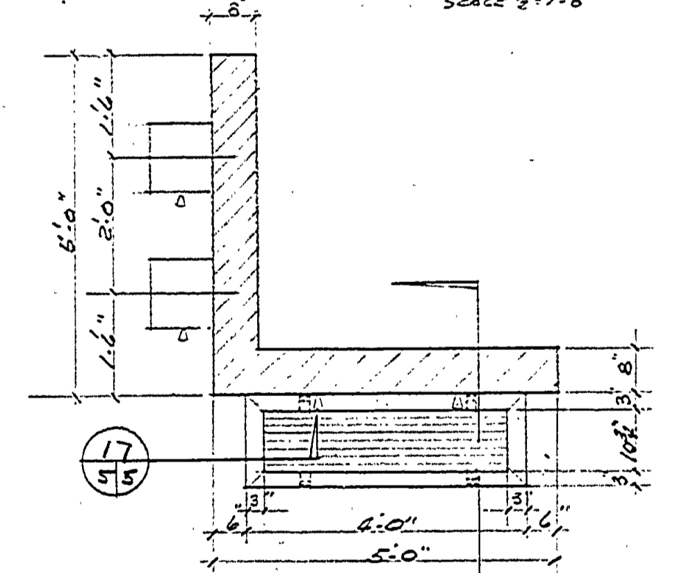
WATER STATION ELEVATIONS
