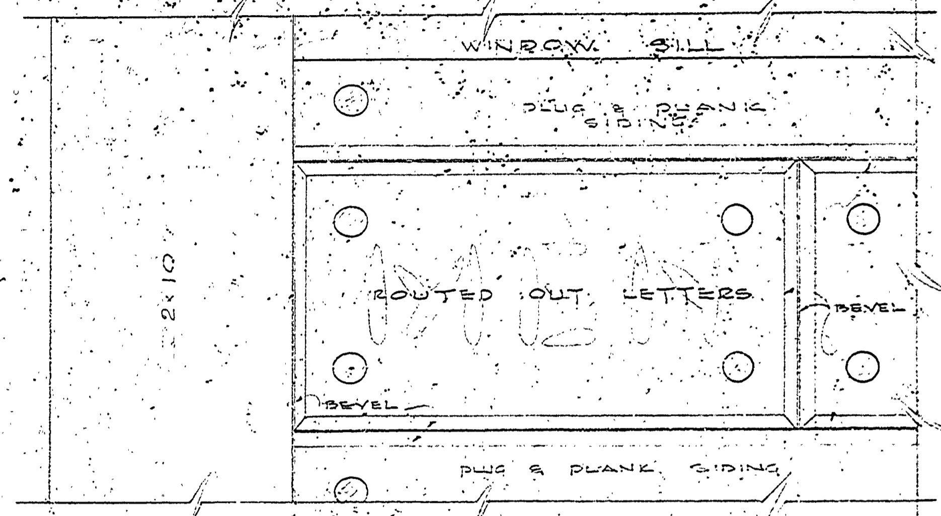
SIGN DET #3 ELEVATION SCALE: 3/8"=1'-0"
