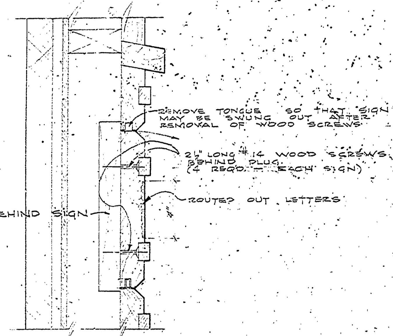
SIGN DET #2 SECT. THROUGH SIGN SCALE: 3/8"=1'-0"
