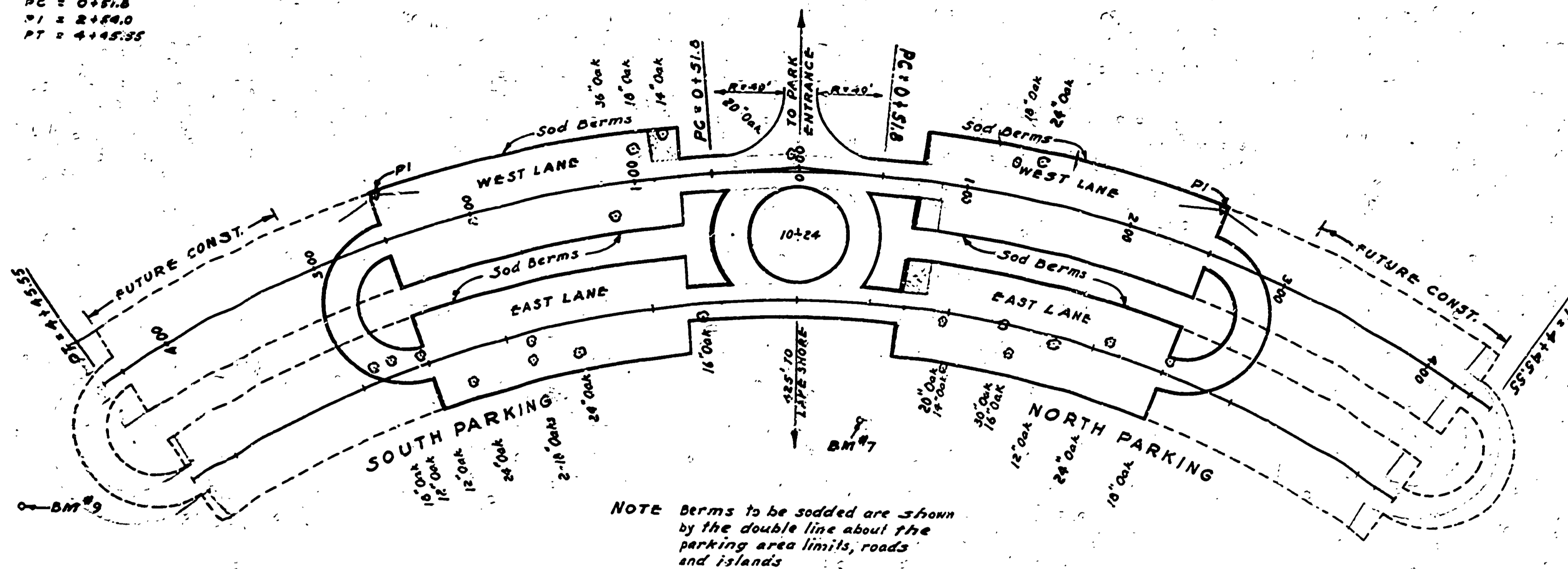
PARKING AREA SCALE - 1" = 50'
