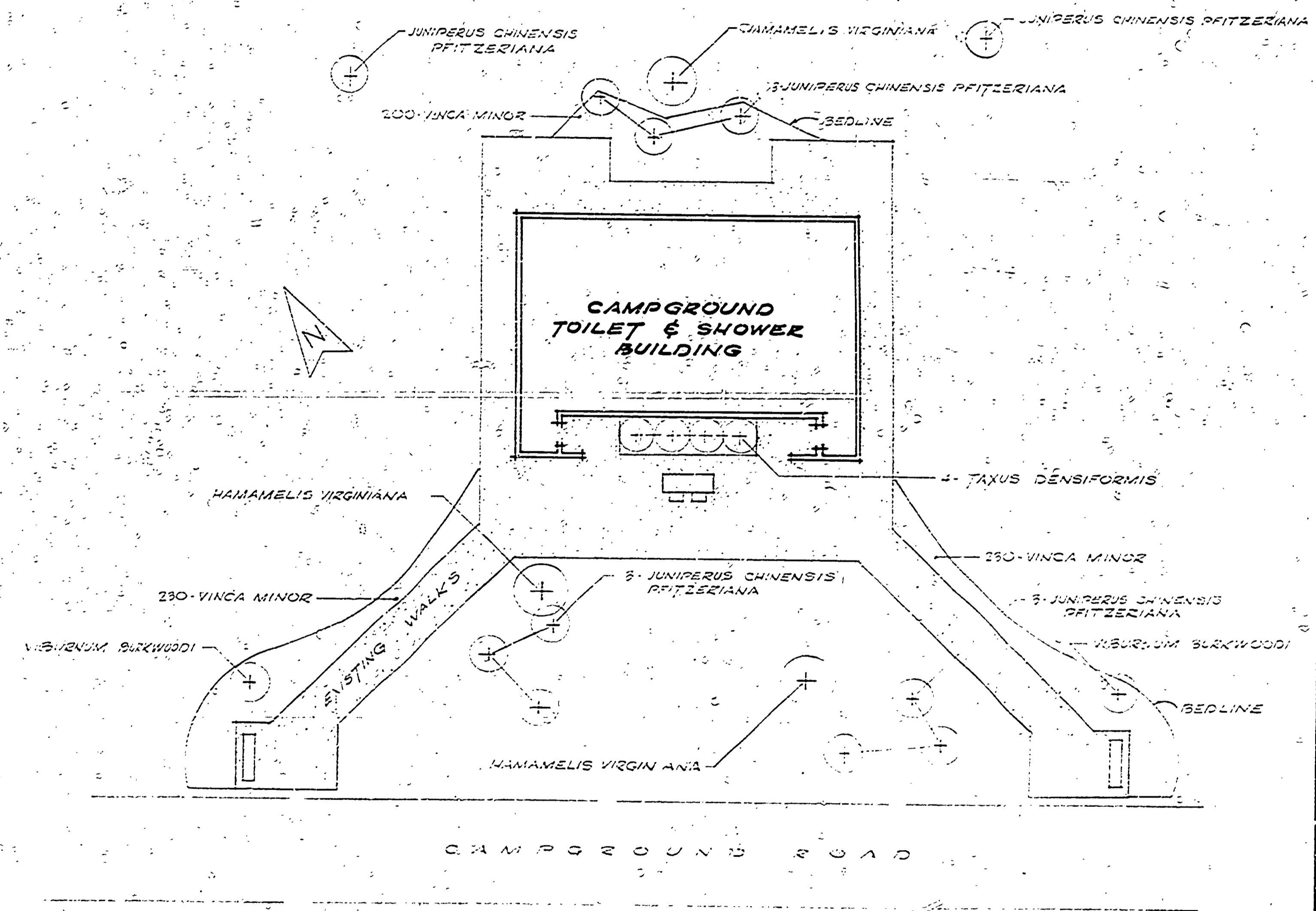
PLAN VIEW HOEFFT STATE PARK SCALE 1" = 10'
