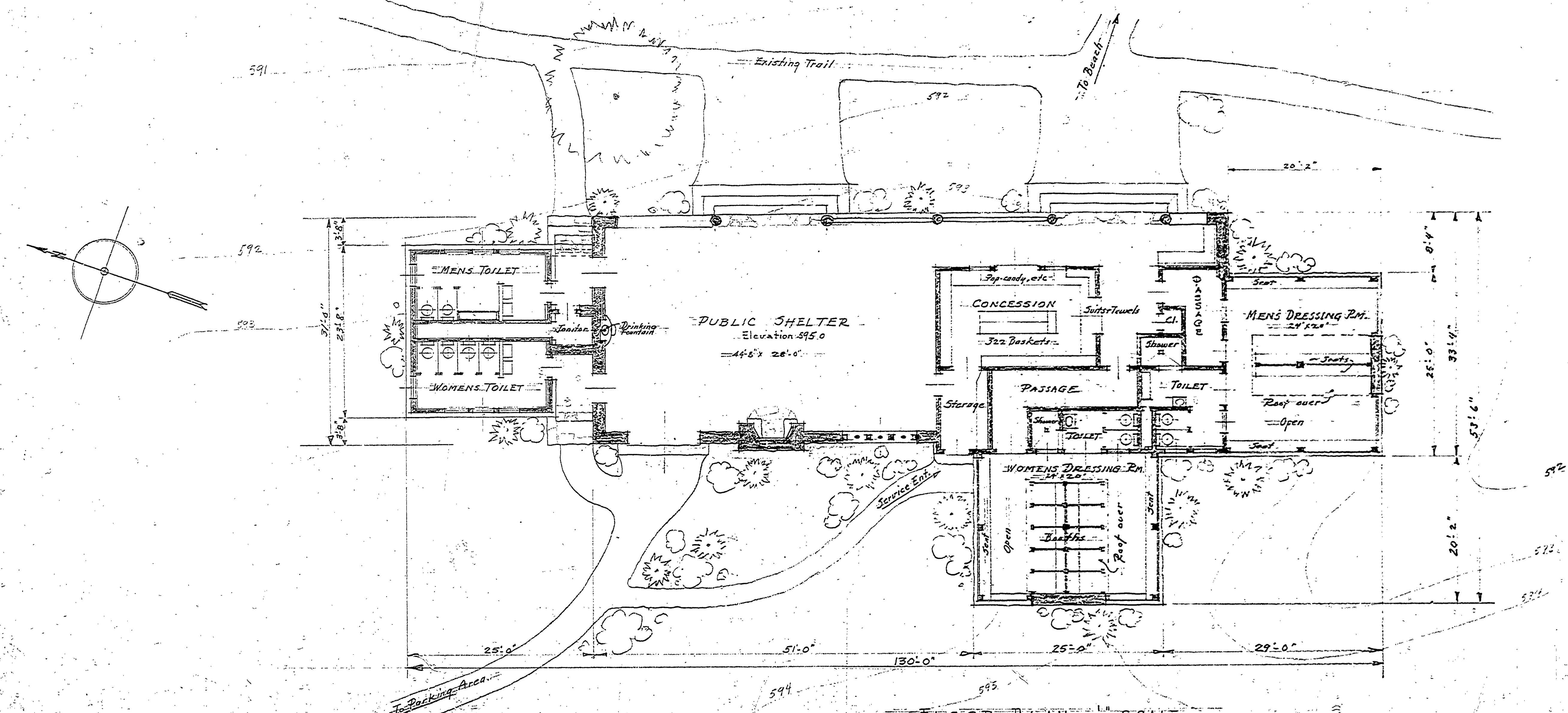
FLOOR PLAN 1/2" SCALE
